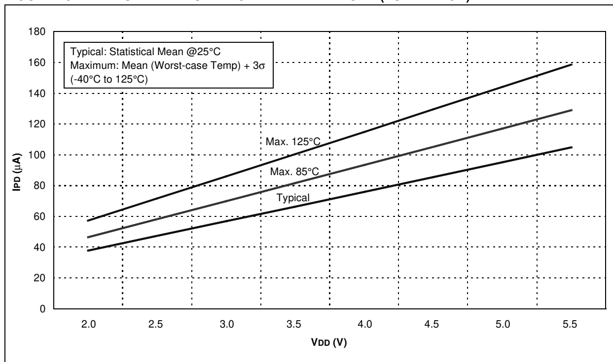
FIGURE 15-22: CVREF IPD vs. VDD OVER TEMPERATURE (LOW RANGE)
