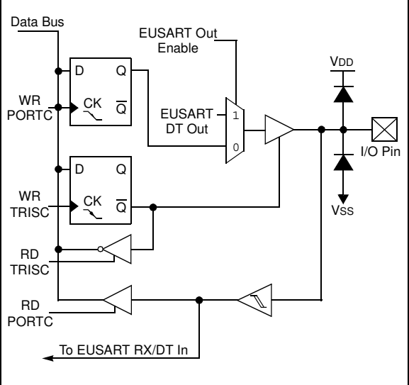
FIGURE 4-10: BLOCK DIAGRAM OF RC5 PIN
