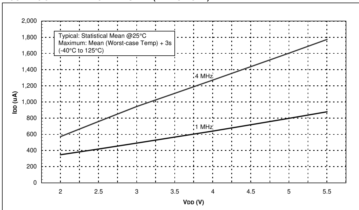
FIGURE 15-8: MAXIMUM I_{DD} vs. V_{DD} (EXTRC MODE)
