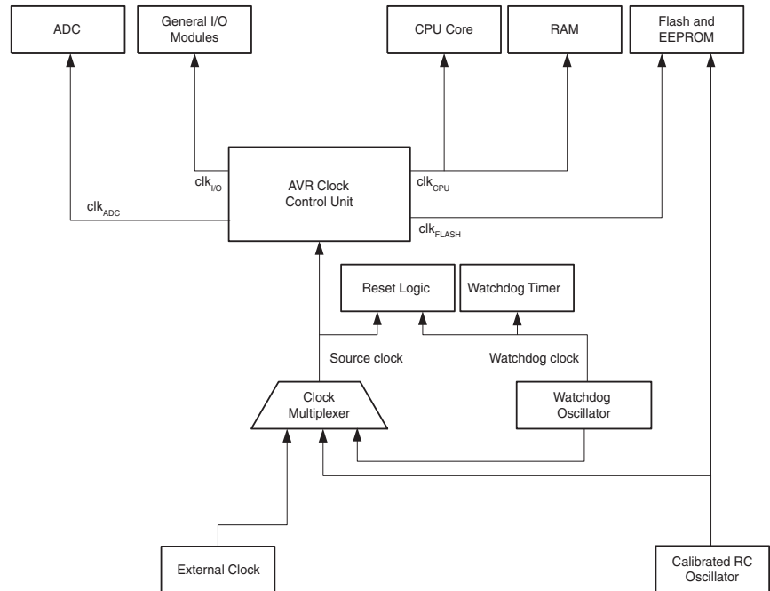
Figure 11. Clock Distribution
