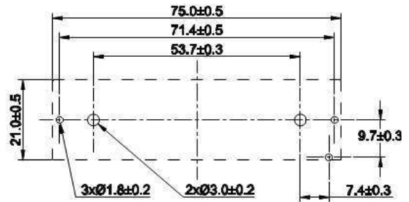
PCB/MOUNTING LAYOUT
