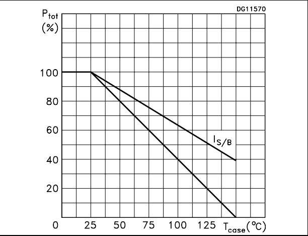
Figure 3. Derating
