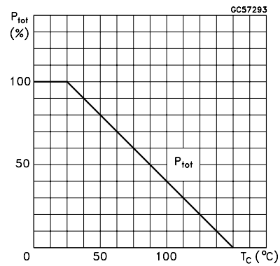
Figure 3. Derating curves
