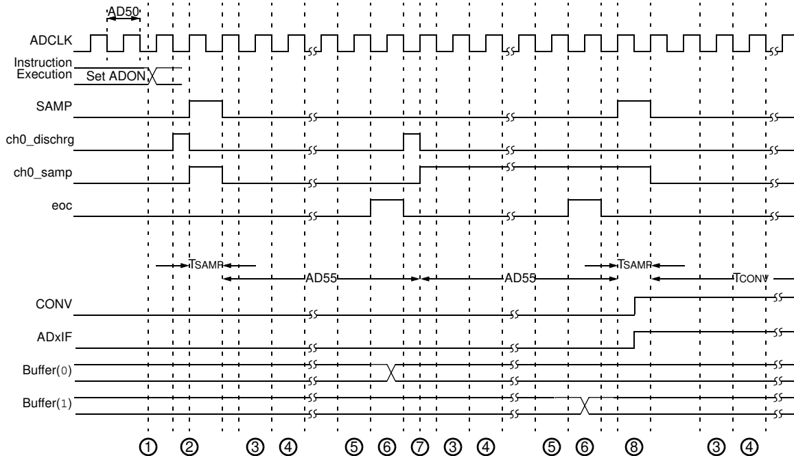
FIGURE 31-20: A/D CONVERSION (10-BIT MODE) TIMING CHARACTERISTICS (CHPS<1:0> = 01, ASAM = 1, SSRC<2:0> = 111, SAMC<4:0> = 00001)
