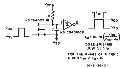
Fig. 17 - Monostable multivibrator.
