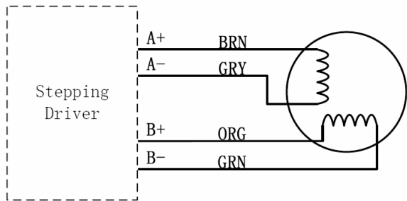
Figure 2: Wiring diagram
