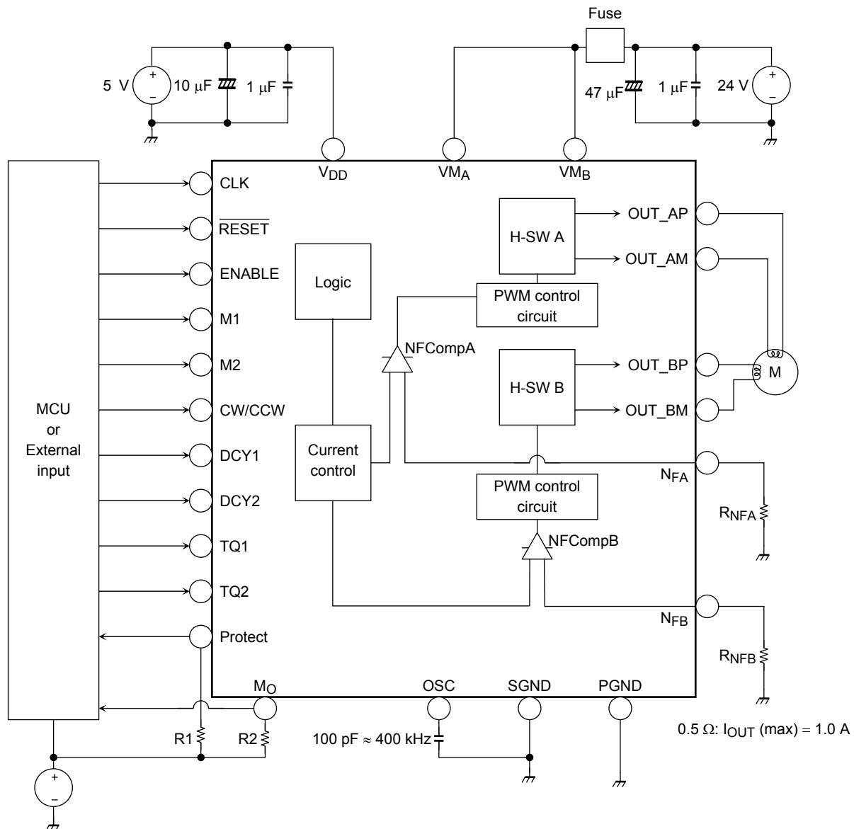
Application Circuit Example
