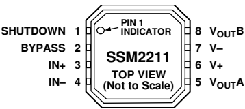
Figure 3. 8-Lead LFCSP_VD Pin Configuration (CP-8-2)
