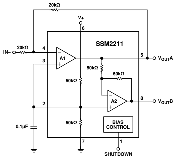
Figure 41. Simplified Schematic
