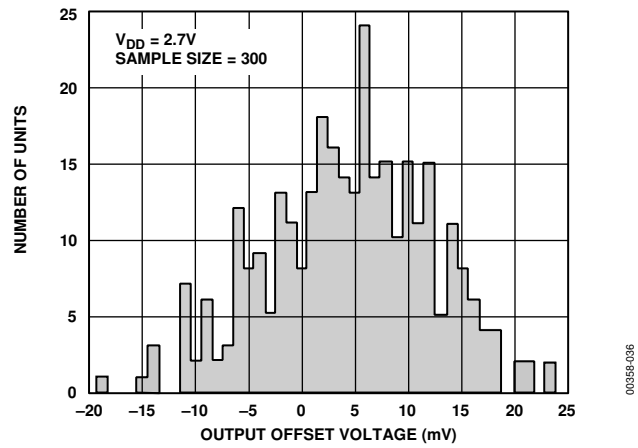
Figure 36. Output Offset Voltage Distribution
