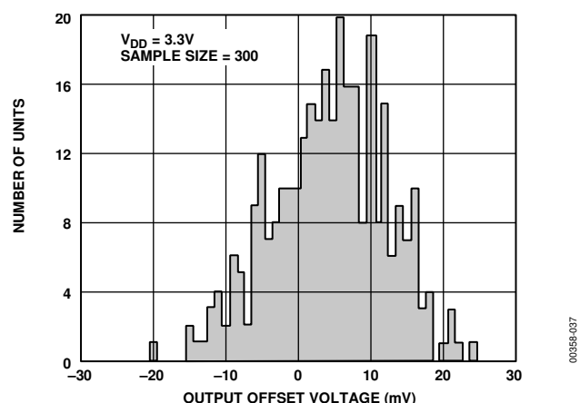
Figure 37. Output Offset Voltage Distribution
