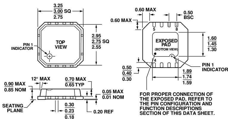
Figure 51. 8-Lead Lead Frame Chip Scale Package [LFCSP_VD] 3 mm × 3 mm Body, Very Thin, Dual Lead (CP-8-2)
