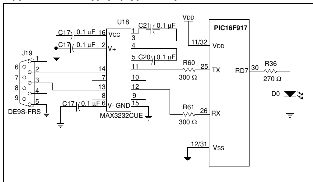
FIGURE 2-17: PROJECT 8: SCHEMATIC
