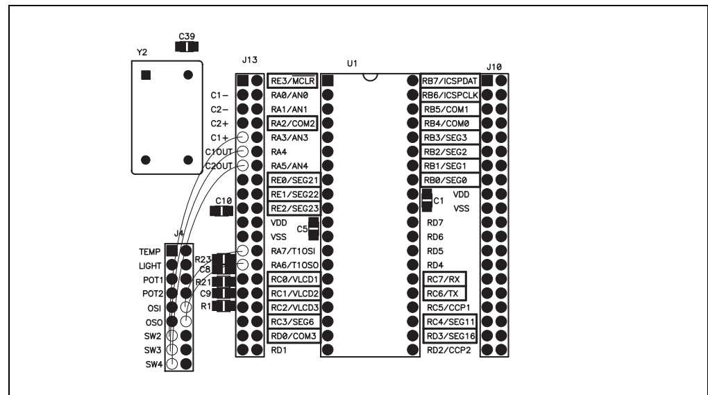
FIGURE 2-8: PROJECT 4: JUMPER DIAGRAM
