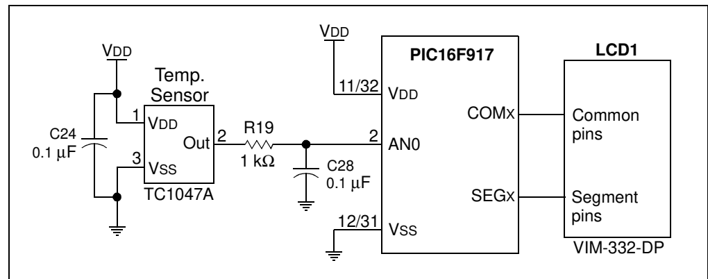
FIGURE 2-7: PROJECT 3: SCHEMATIC
