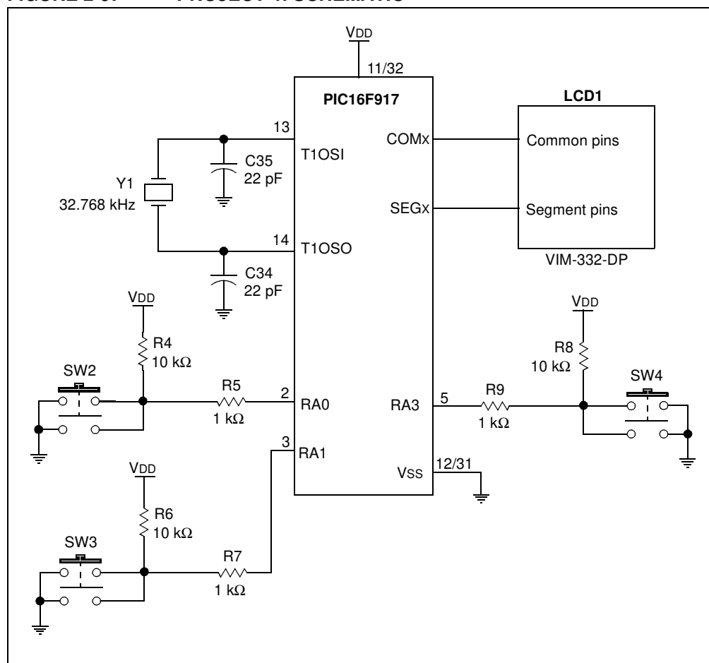
FIGURE 2-9: PROJECT 4: SCHEMATIC
