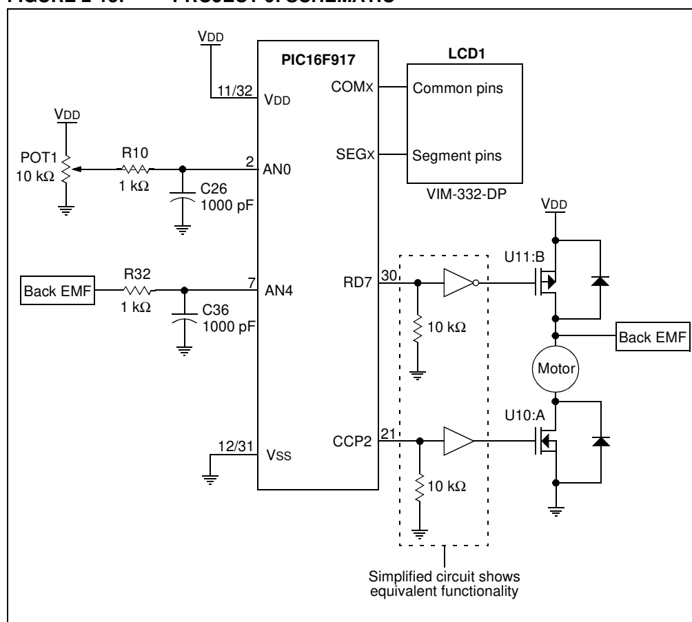
FIGURE 2-13: PROJECT 6: SCHEMATIC
