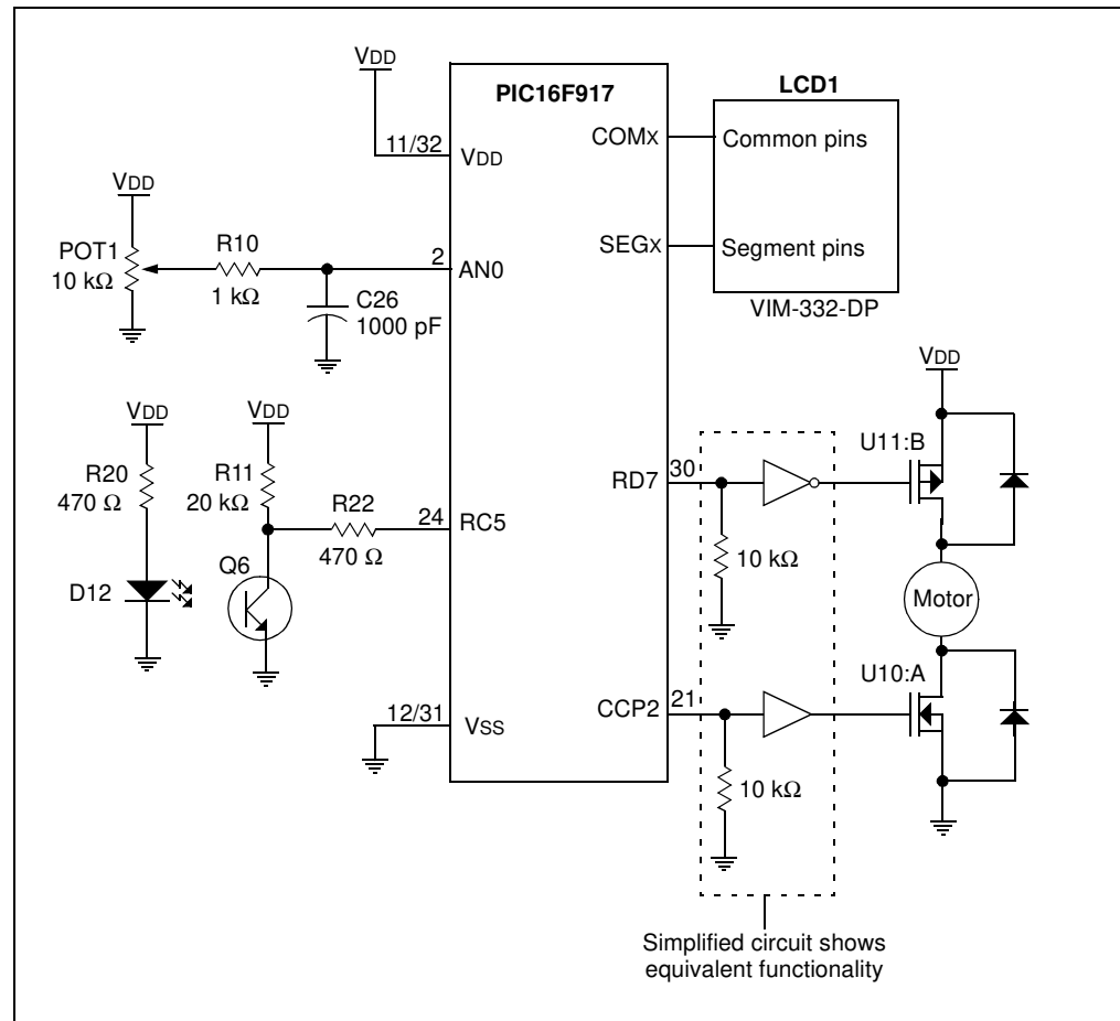
FIGURE 2-11: PROJECT 5: SCHEMATIC
