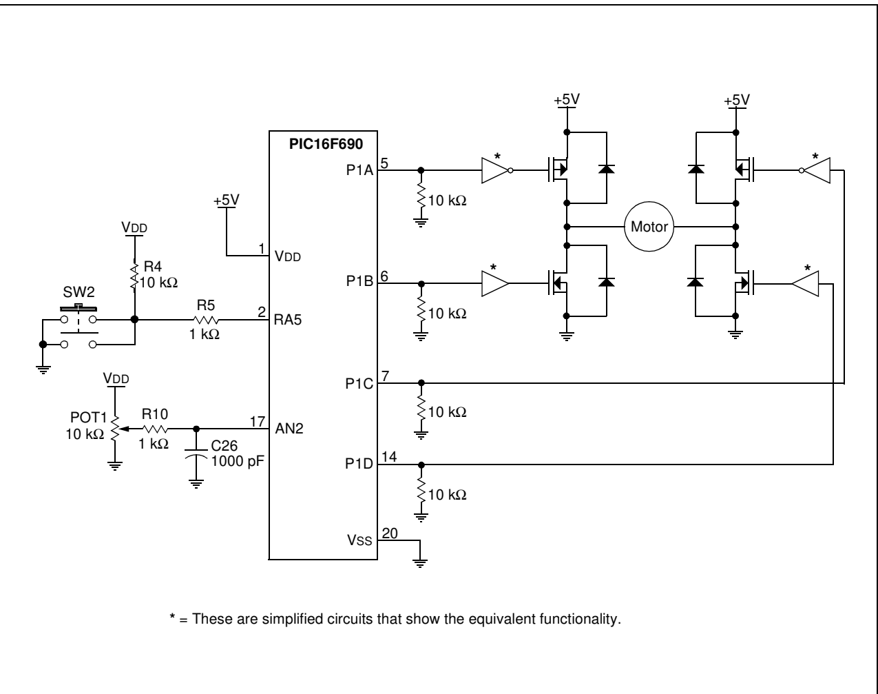
FIGURE 2-20: PROJECT 9: SCHEMATIC
