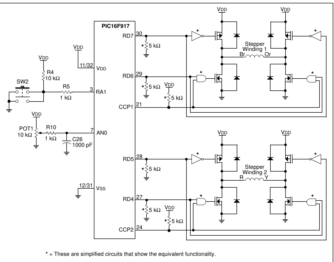
FIGURE 2-15: PROJECT 7: SCHEMATIC
