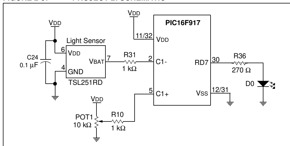
FIGURE 2-5: PROJECT 2: SCHEMATIC
