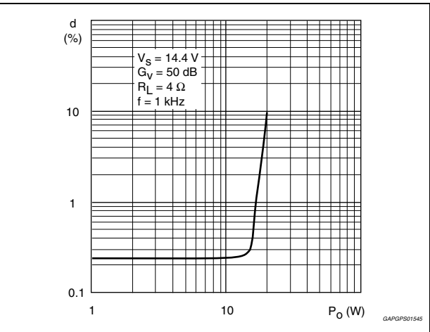
Figure 6. Distortion vs. output power ( R_L = 4\ \Omega )
