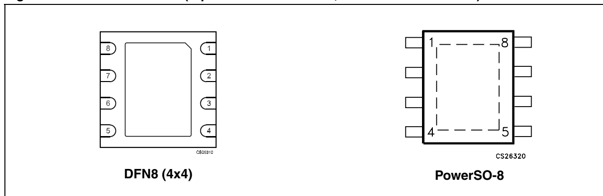
Figure 2. Pin connections (top view for PowerSO-8, bottom view for DFN8)
