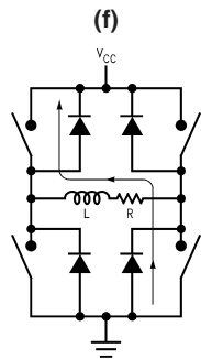
FIGURE 1. Chopper Amplifier Chopping States: Full V_{CC} Applied Across the Winding (a) and (d), Shorted Winding (b) and (e), Winding Current Decays During a Change in the Direction of the Winding Current (c) and (f), and the Chopped Winding Current (g)
