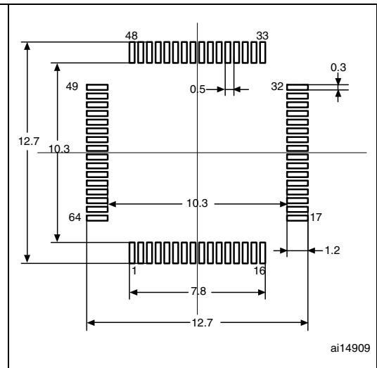
Figure 44. Recommended footprint (1)(2)
