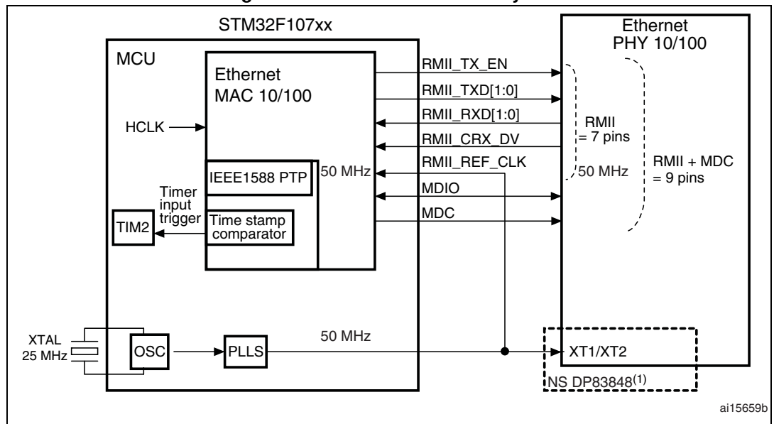
Figure 52. RMI with a 25 MHz crystal
