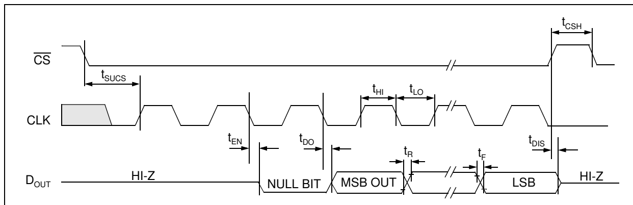
FIGURE 1-1: Serial Timing.
