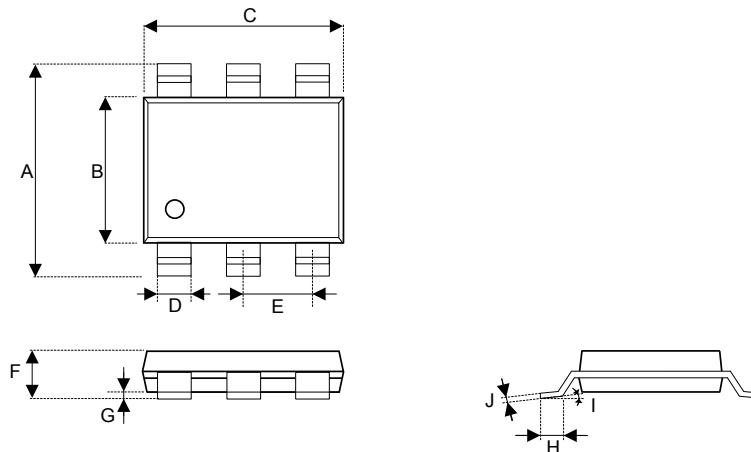
Figure 9.1 TSOT23-6 Packaging 1
