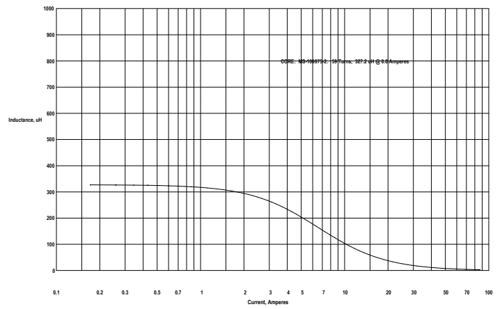
DTMS-27/0,33/2,0
