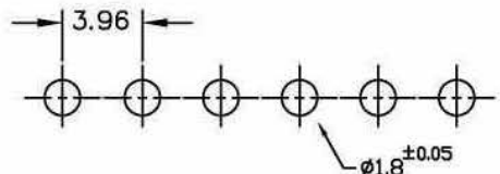
PCB LAYOUT COMPONENT SIDE
