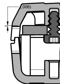
SECTION U-U SCALE 3.000
