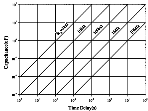
Figure 2. Resistance and Capacitance vs. Time delay( t d )
