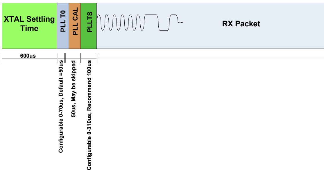
Figure 9. RX Timing
