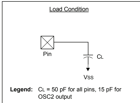
FIGURE 25-7: LOAD CONDITIONS
