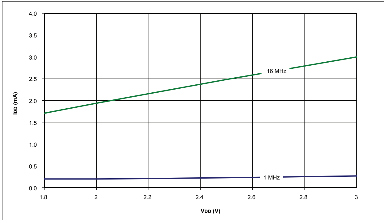
FIGURE 26-9: PIC18LF1XK22 TYPICAL PRI_RUN I DD (EC)
