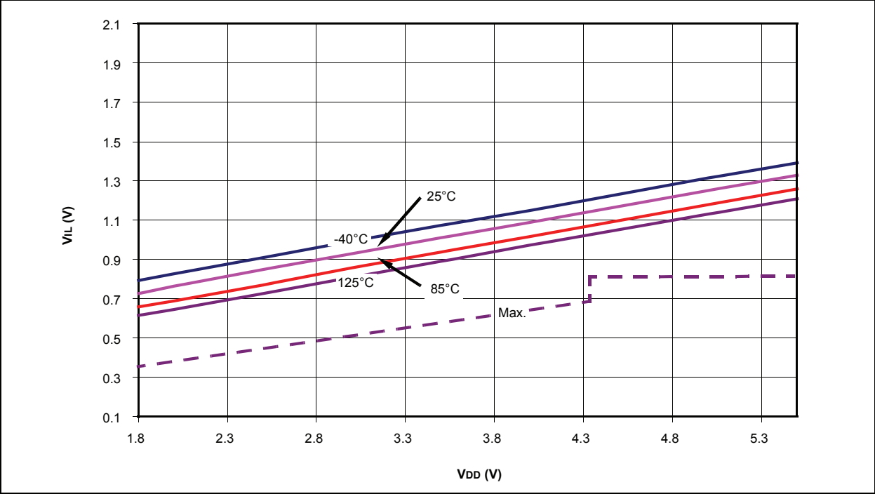
FIGURE 26-24: PIC18(L)F1XK22 SCHMITT BUFFER TYPICAL V_{IL}
