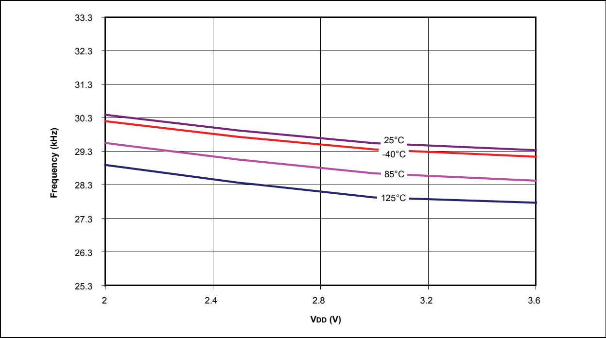
FIGURE 26-28: PIC18LF1XK22 TYPICAL LF-INTOSC FREQUENCY (MAX./MIN. = 31.25 kHz ± 15%)
