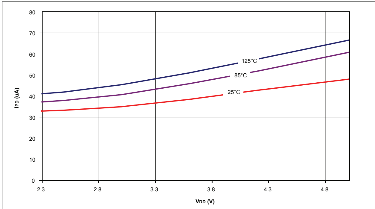
FIGURE 26-14: PIC18F1XK22 TYPICAL I_{PD} FOR COMPARATOR VOLTAGE REFERENCE
