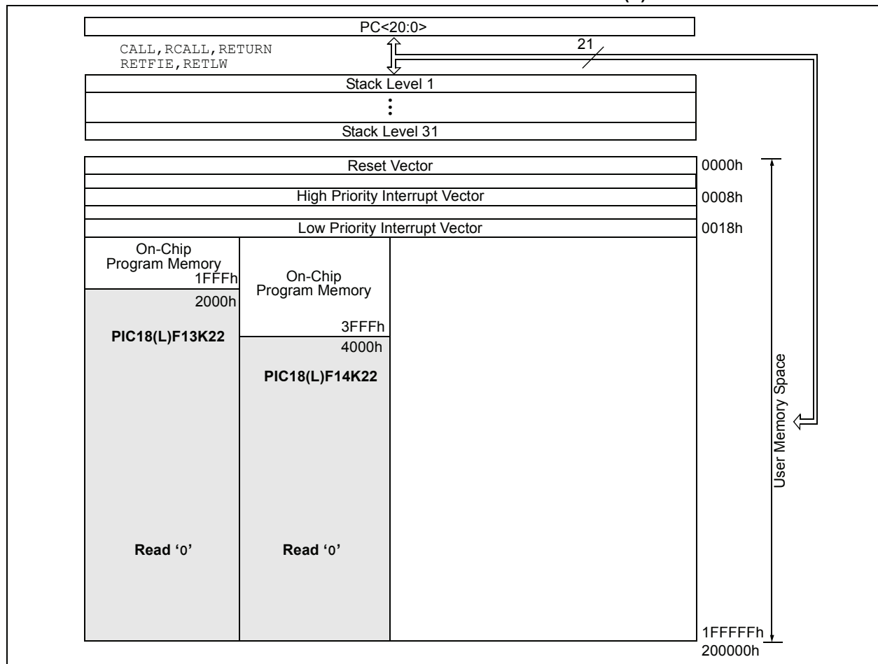
FIGURE 3-1: PROGRAM MEMORY MAP AND STACK FOR PIC18(L)F1XK22 DEVICES
