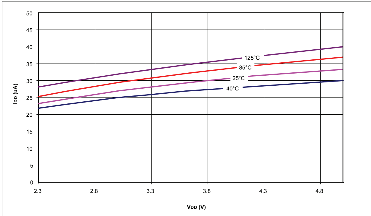
FIGURE 26-17: PIC18F1XK22 TYPICAL RC_RUN 31 kHz I DD
