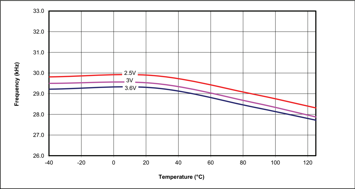
FIGURE 26-28: PIC18LF1XK22 TYPICAL LF-INTOSC FREQUENCY (MAX./MIN. = 31.25 kHz ± 15%)
