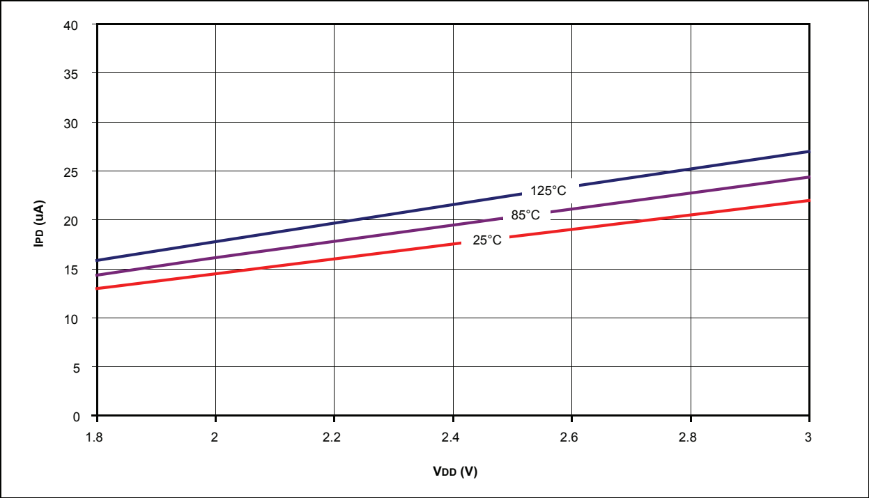
FIGURE 26-4: PIC18LF1XK22 TYPICAL I PD FOR COMPARATOR VOLTAGE REFERENCE
