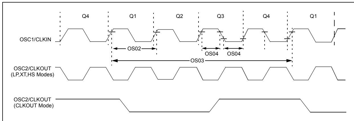
FIGURE 25-8: CLOCK TIMING
