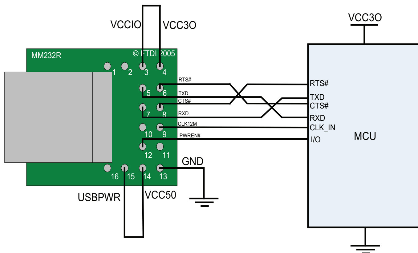
Figure 8 - Bus Powered with 3.3V Logic Drive
