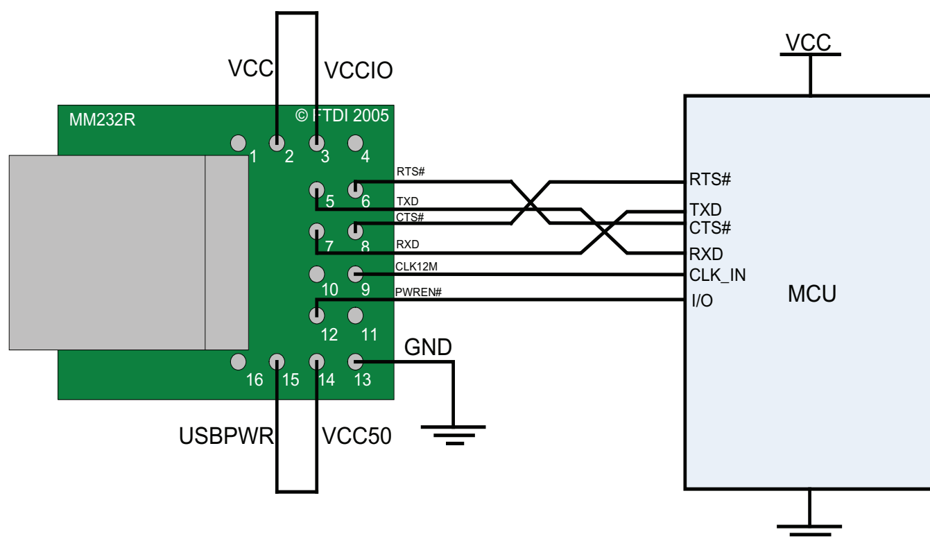
Figure 5 - Bus Powered Configuration
