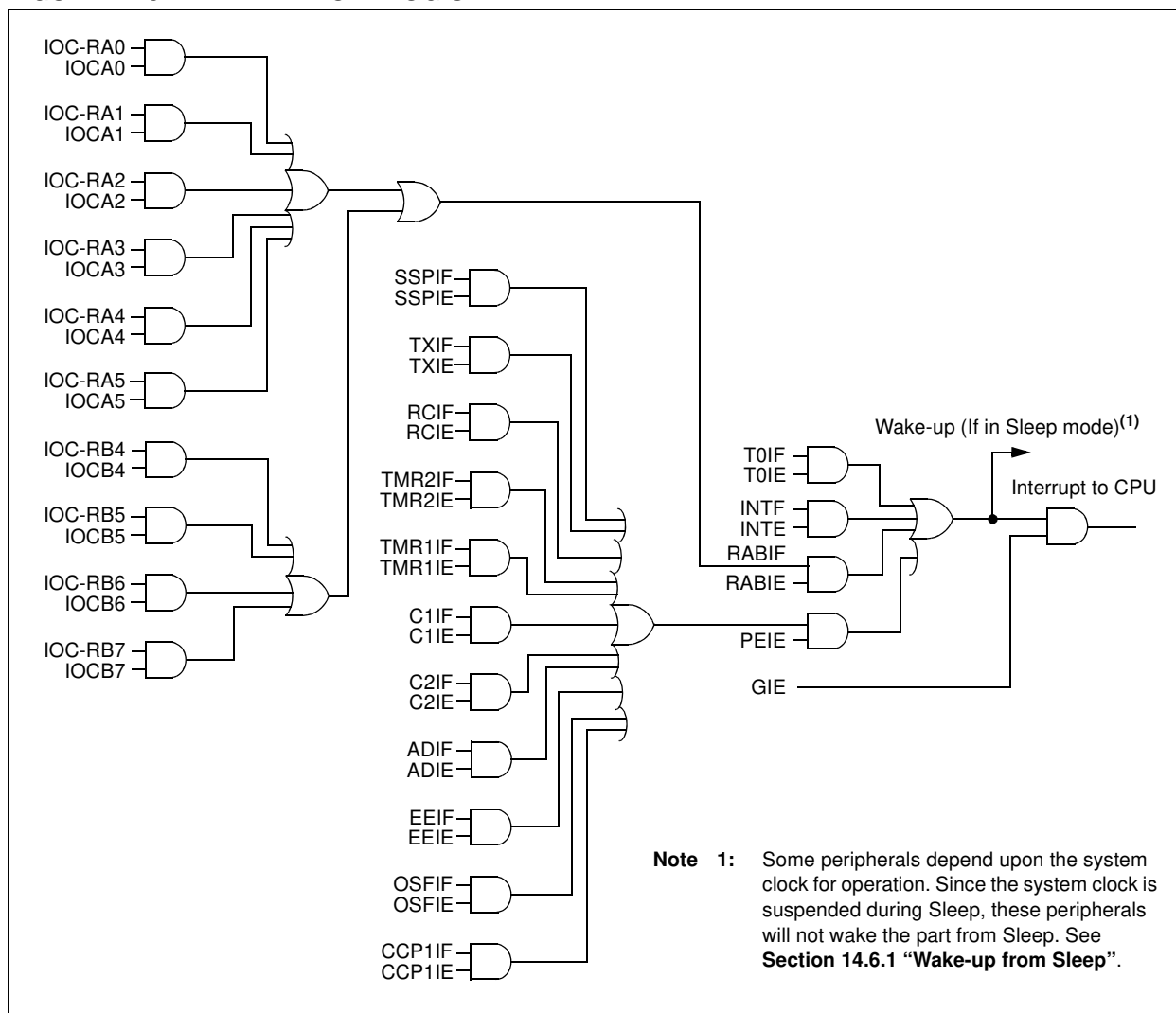
FIGURE 14-6: INTERRUPT LOGIC
