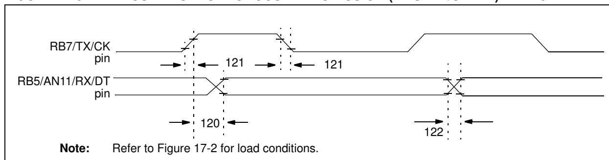
FIGURE 17-9: EUSART SYNCHRONOUS TRANSMISSION (MASTER/SLAVE) TIMING
