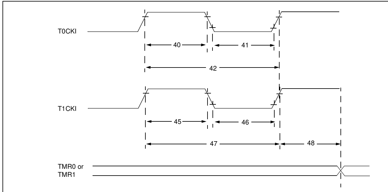
FIGURE 17-7: TIMER0 AND TIMER1 EXTERNAL CLOCK TIMINGS
