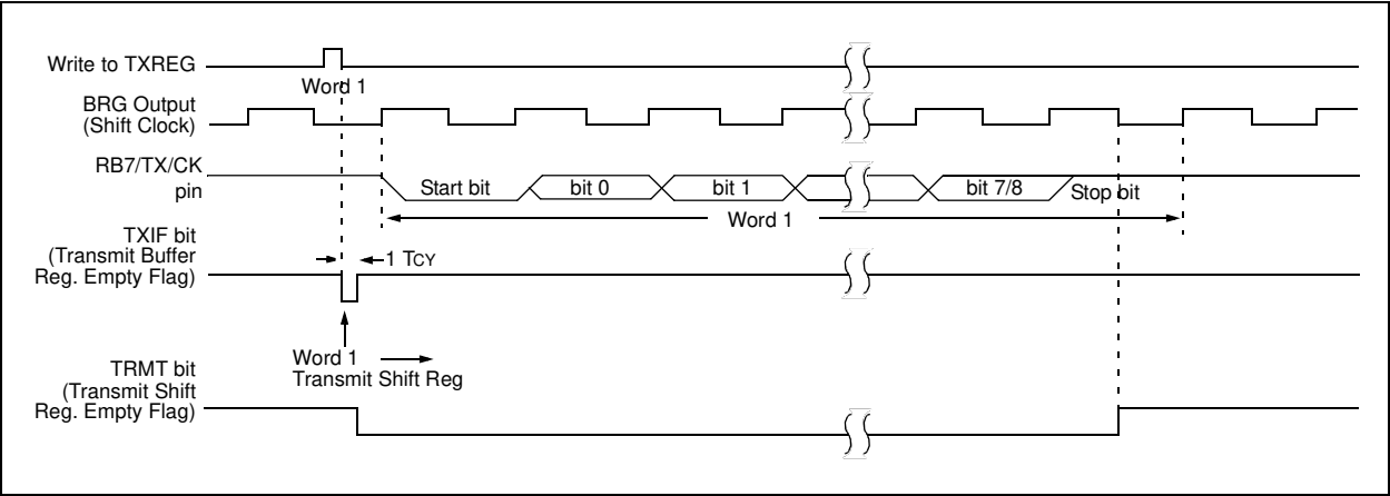
FIGURE 12-4: ASYNCHRONOUS TRANSMISSION (BACK-TO-BACK)
