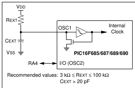
FIGURE 3-6: RCIO MODE
