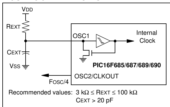
FIGURE 3-5: RC MODE
