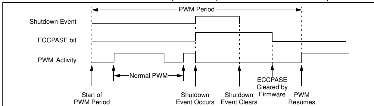
FIGURE 11-15: PWM AUTO-SHUTDOWN (PRSEN = 0, AUTO-RESTART DISABLED)
