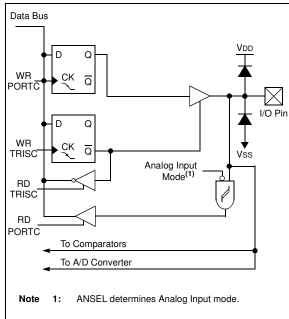
FIGURE 4-11: BLOCK DIAGRAM OF RC0 AND RC1
