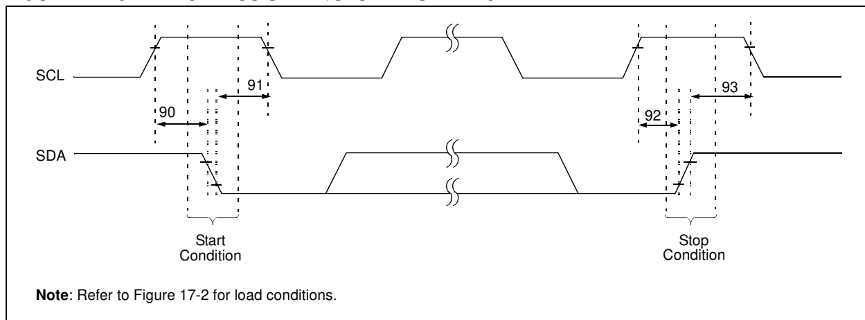
FIGURE 17-15: I²C™ BUS START/STOP BITS TIMING
