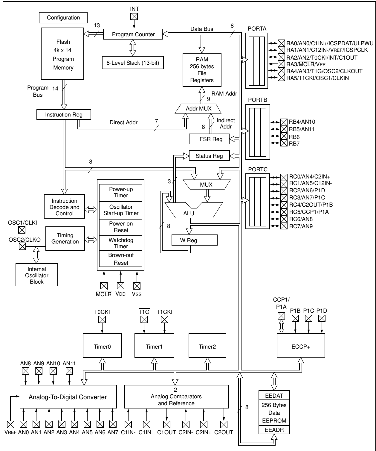
FIGURE 1-1: PIC16F685 BLOCK DIAGRAM
