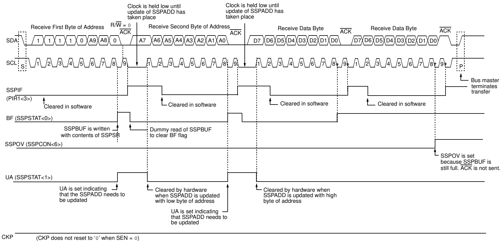
FIGURE 13-11: I 2 C™ SLAVE MODE TIMING (TRANSMISSION, 10-BIT ADDRESS)
