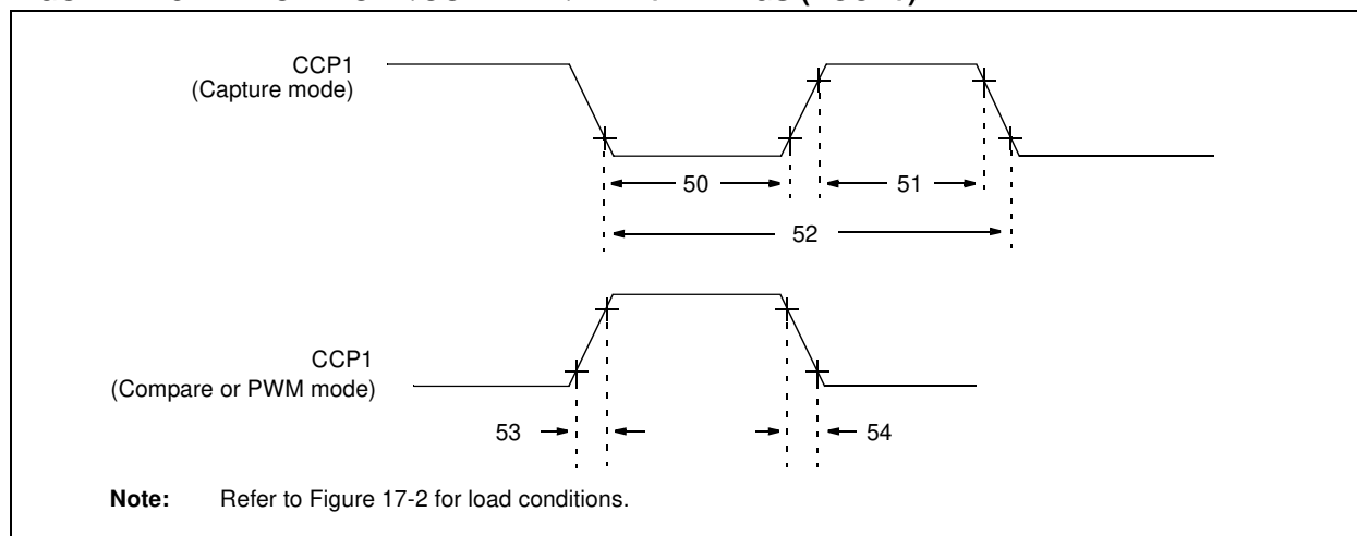
FIGURE 17-8: CAPTURE/COMPARE/PWM+ TIMINGS (ECCP+)
