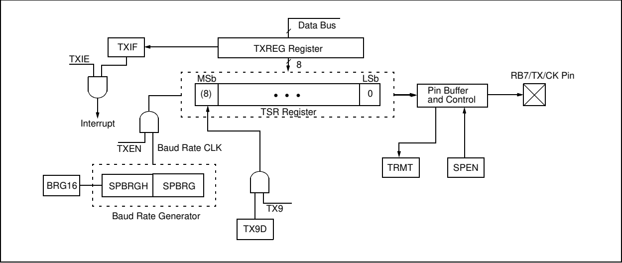
FIGURE 12-3: ASYNCHRONOUS TRANSMISSION
