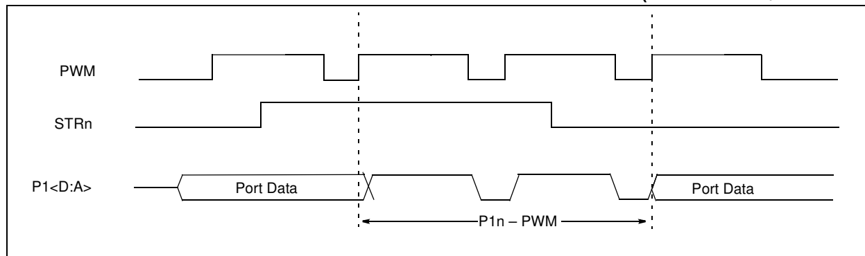
FIGURE 11-13: STEERING EVENT AT BEGINNING OF INSTRUCTION (STRSYNC = 1)
