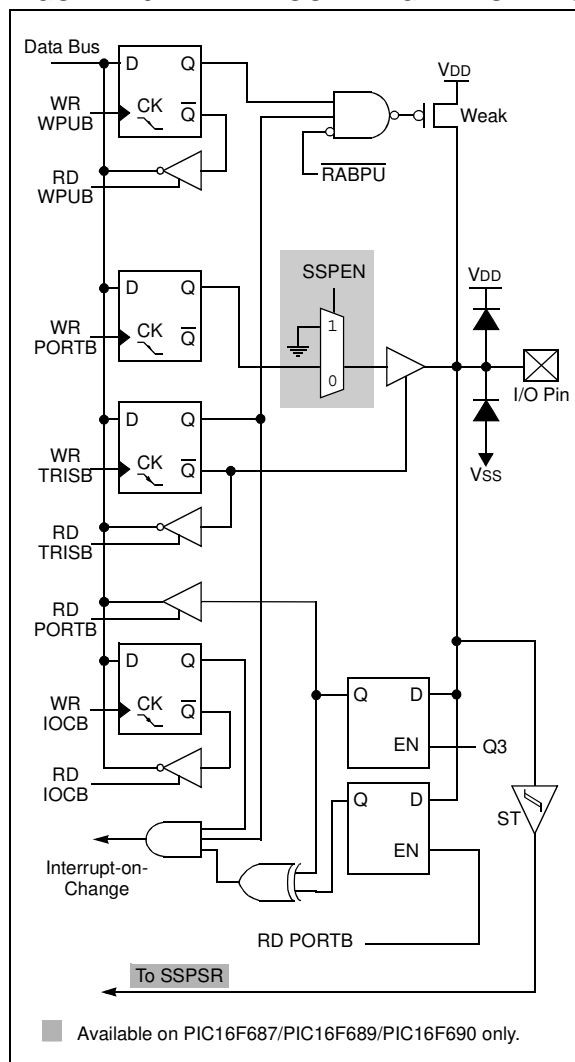
FIGURE 4-9: BLOCK DIAGRAM OF RB6
