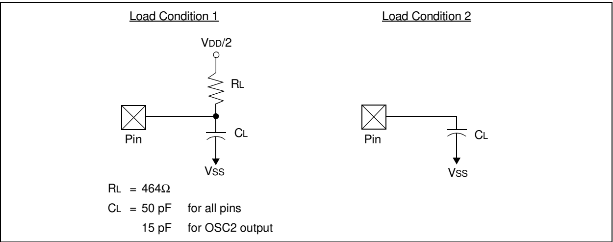
FIGURE 17-2: LOAD CONDITIONS
