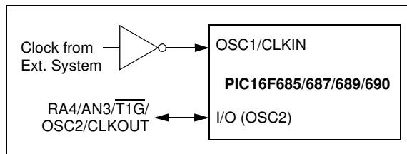
FIGURE 3-2: EXTERNAL CLOCK (EC) MODE OPERATION
