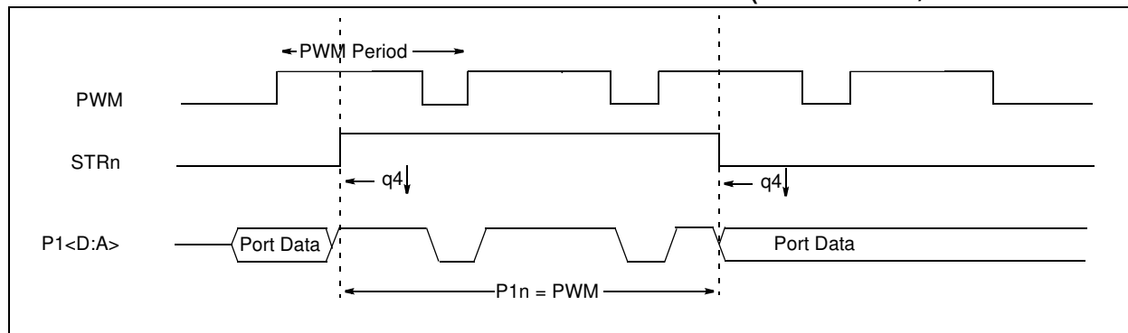
FIGURE 11-12: STEERING EVENT AT END OF INSTRUCTION (STRSYNC = 0)
