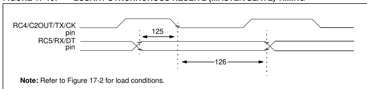
FIGURE 17-10: EUSART SYNCHRONOUS RECEIVE (MASTER/SLAVE) TIMING
