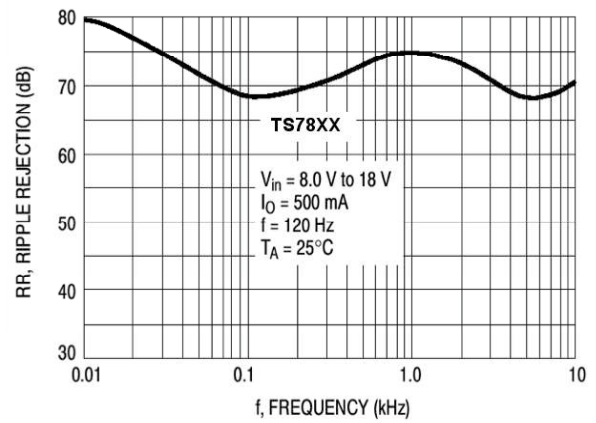
FIGURE 8 – Ripple Rejection v.s. Frequency
