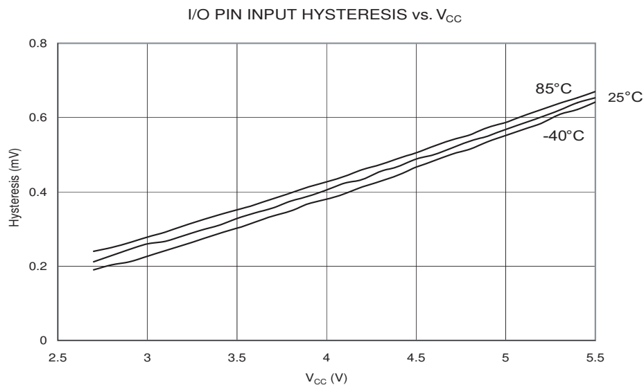
Figure 184. I/O Pin Input Hysteresis vs. V_{CC}
