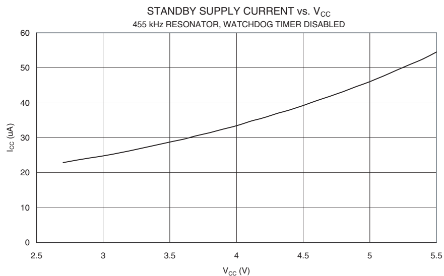
Figure 166. Standby Supply Current vs. V_{CC} (455 kHz Resonator, Watchdog Timer Disabled)
