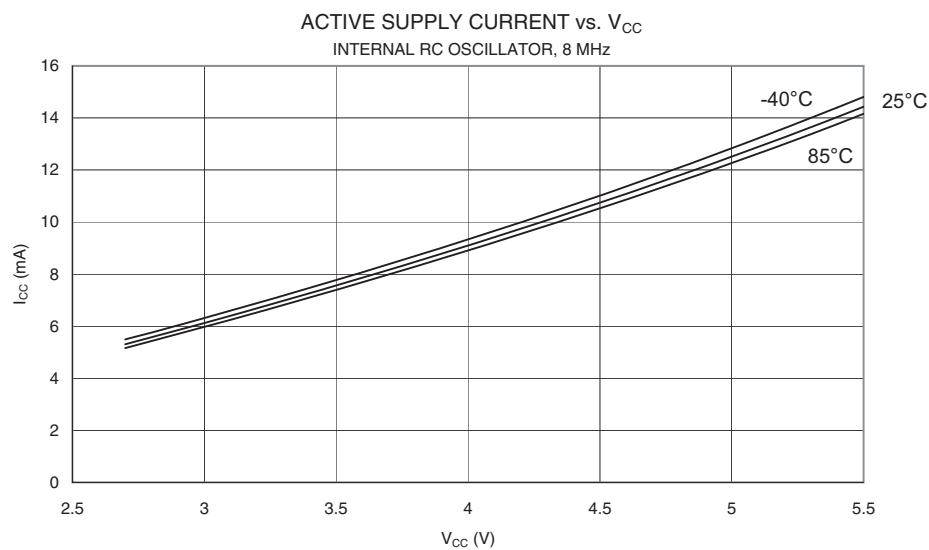
Figure 151. Active Supply Current vs. V_{CC} (Internal RC Oscillator, 8 MHz)
