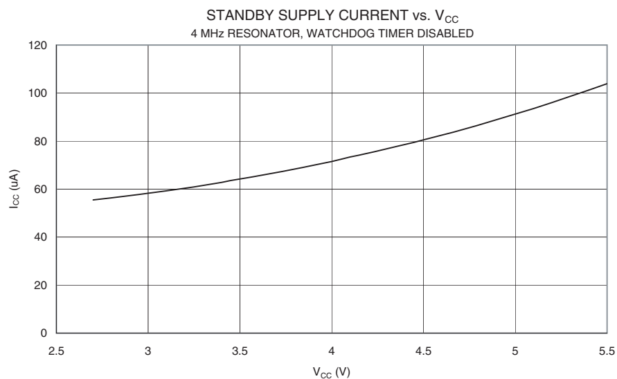
Figure 170. Standby Supply Current vs. V_{CC} (4 MHz Resonator, Watchdog Timer Disabled)
