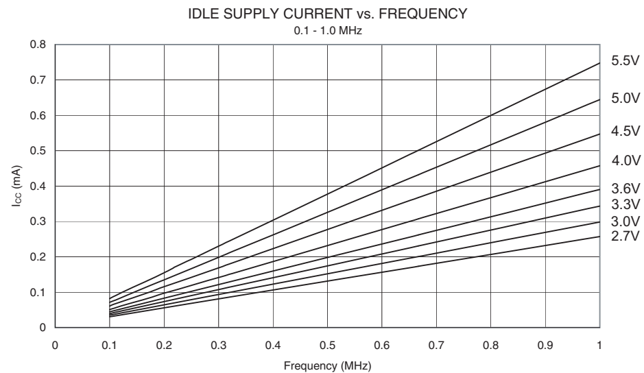
Figure 156. Idle Supply Current vs. Frequency (0.1 - 1.0 MHz)
