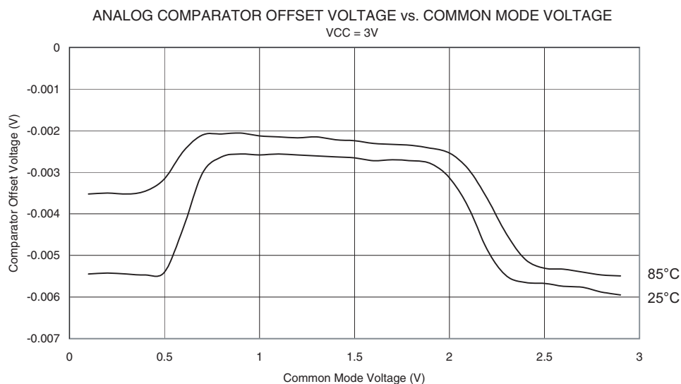
Figure 192. Analog Comparator Offset Voltage vs. Common Mode Voltage ( V_{CC} = 3V )
