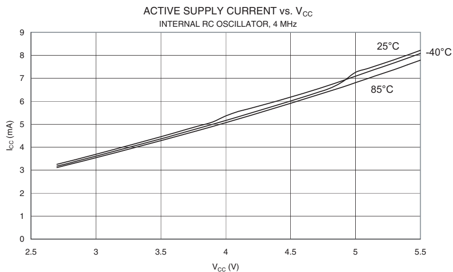
Figure 152. Active Supply Current vs. V_{CC} (Internal RC Oscillator, 4 MHz)
