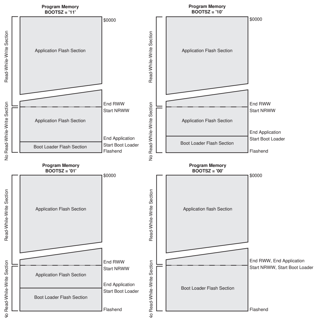
Figure 125. Memory Sections (1)
