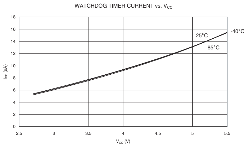
Figure 210. Watchdog Timer Current vs. V_{CC}
