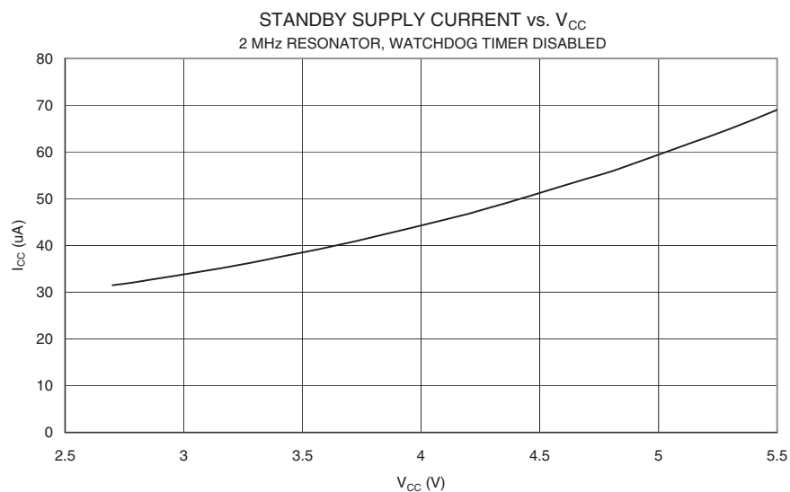
Figure 168. Standby Supply Current vs. V_{CC} (2 MHz Resonator, Watchdog Timer Disabled)
