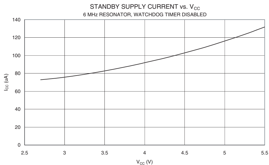
Figure 172. Standby Supply Current vs. V_{CC} (6 MHz Resonator, Watchdog Timer Disabled)
