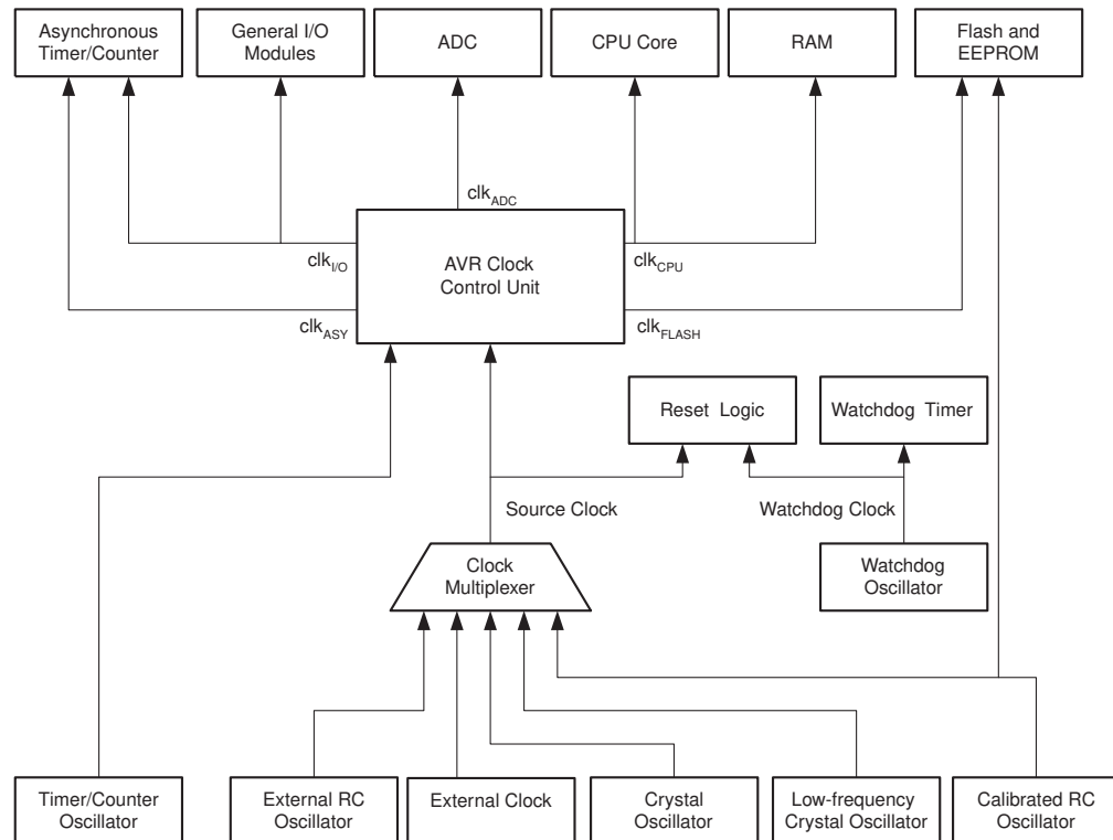
Figure 11. Clock Distribution
