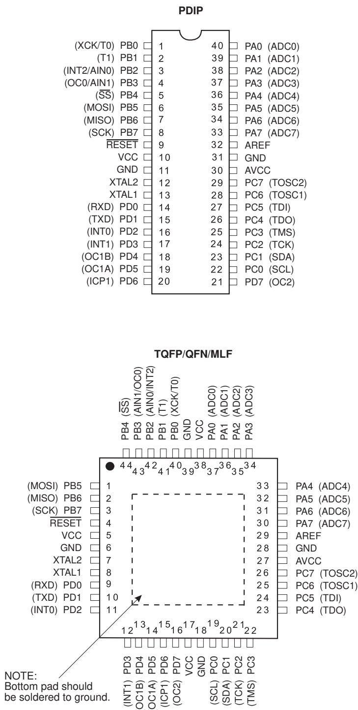
Figure 1. Pinout ATmega16
