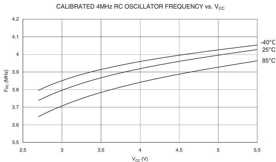
Figure 198. Calibrated 4 MHz RC Oscillator Frequency vs. V_{CC}
