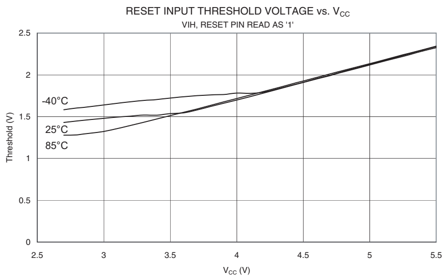
Figure 185. Reset Input Threshold Voltage vs. V_{CC} ( V_{IH} , Reset Pin Read As '1')
