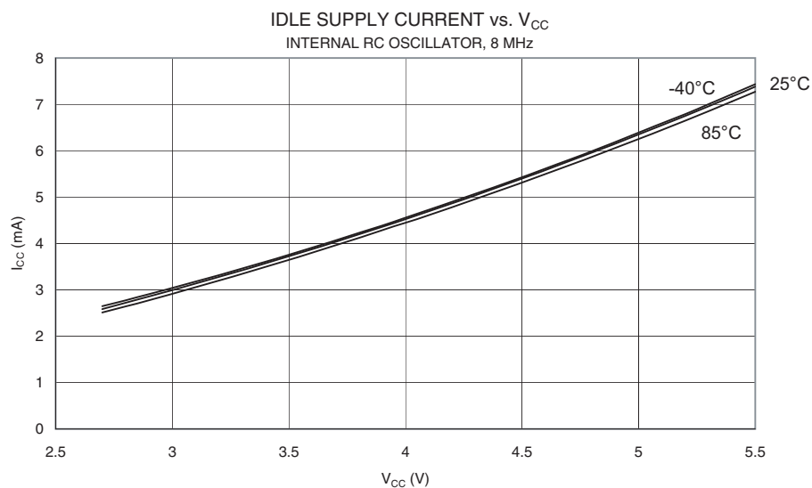
Figure 158. Idle Supply Current vs. V_{CC} (Internal RC Oscillator, 8 MHz)
