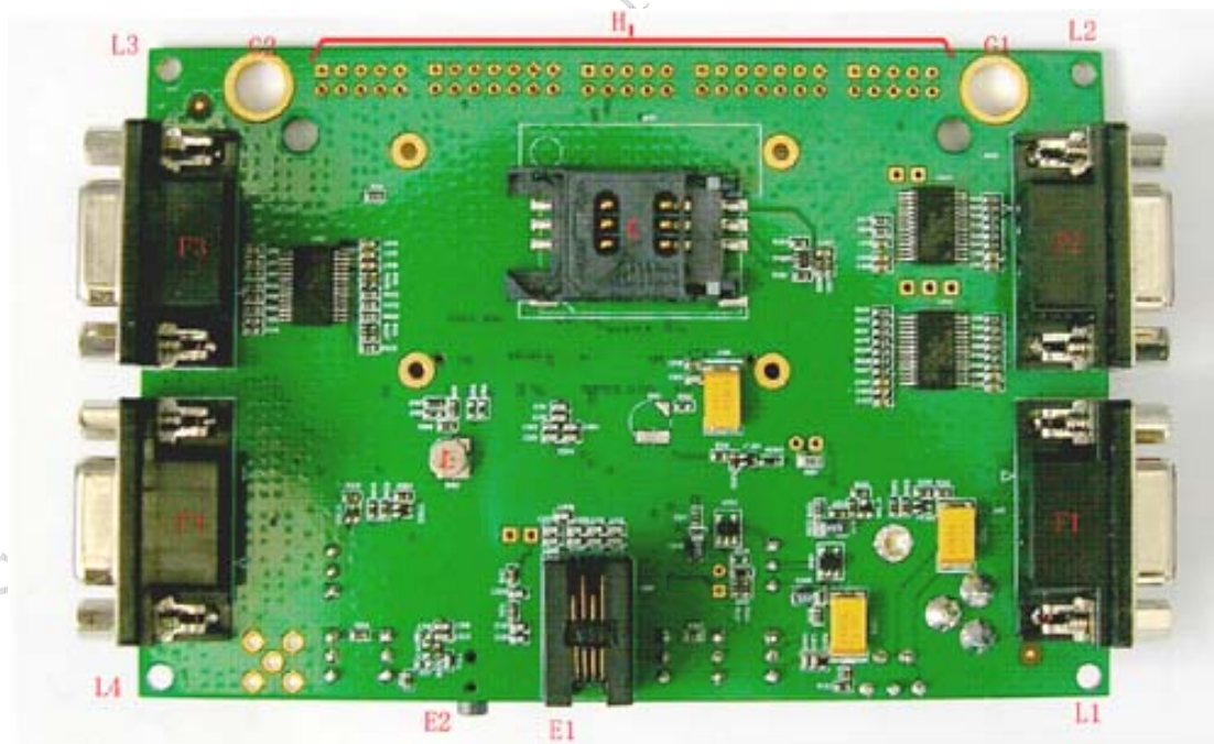
Figure 1: TOP view
