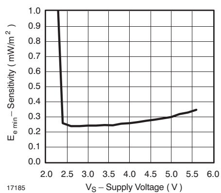
Figure 14. Sensitivity vs. Supply Voltage
