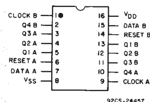
TERMINAL DIAGRAM
