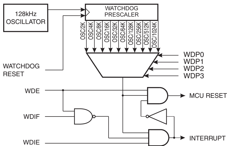
Figure 10-7. Watchdog Timer
