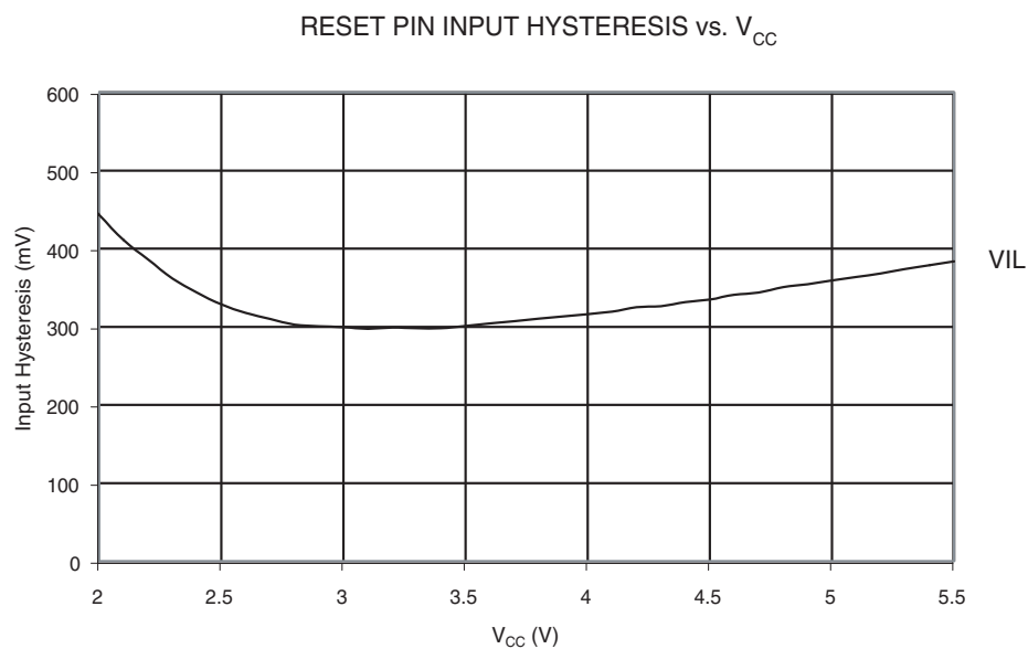
Figure 29-33. Reset Input Pin Hysteresis vs. V_{CC}
