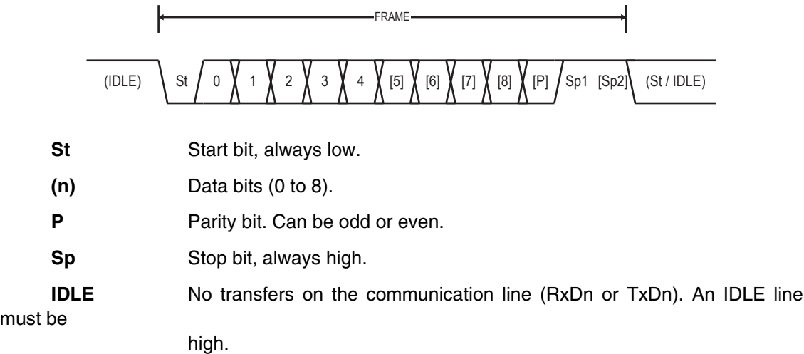
Figure 19-4. Frame Formats
