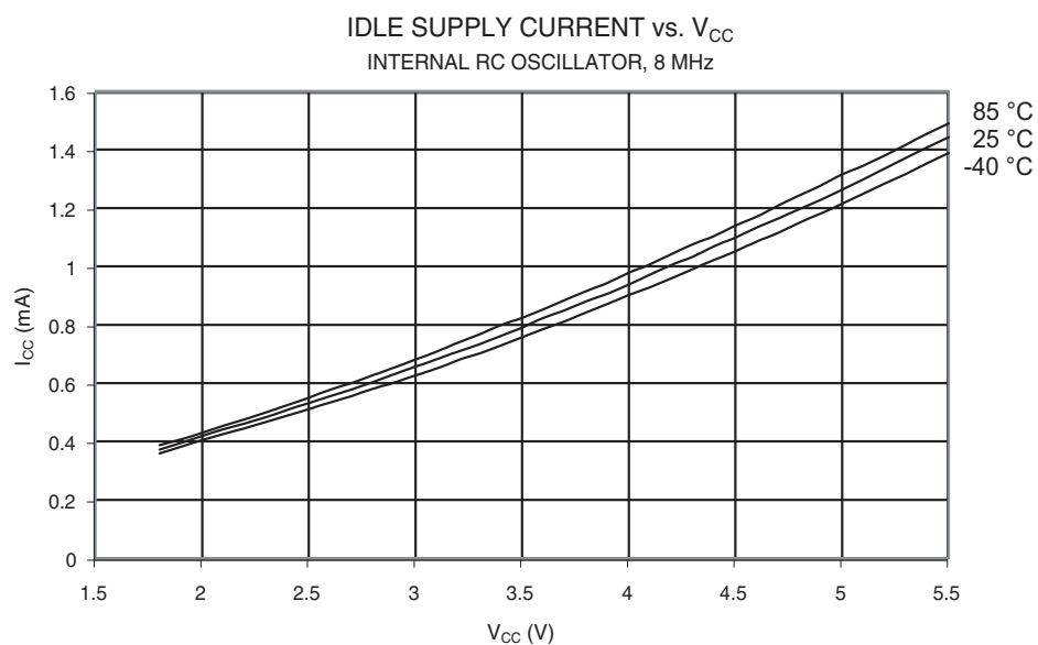
Figure 29-11. Idle Supply Current vs. V_{CC} (Internal RC Oscillator, 8 MHz)
