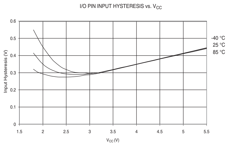
Figure 29-30. I/O Pin Input Hysteresis vs. V_{CC}
