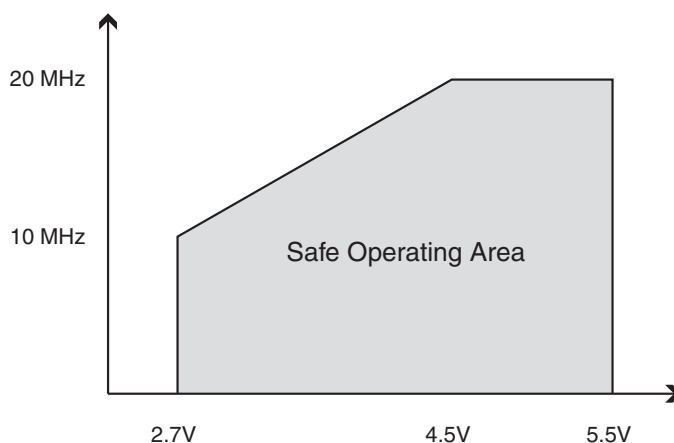
Figure 28-2. Maximum Frequency vs. V_{CC} , ATmega48/88/168
