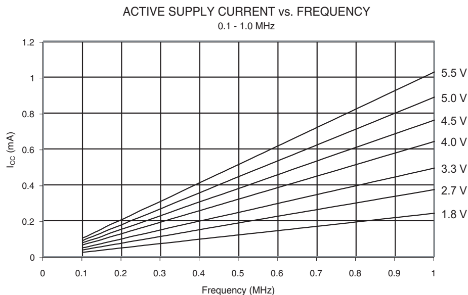
Figure 29-1. Active Supply Current vs. Frequency (0.1 - 1.0 MHz)
