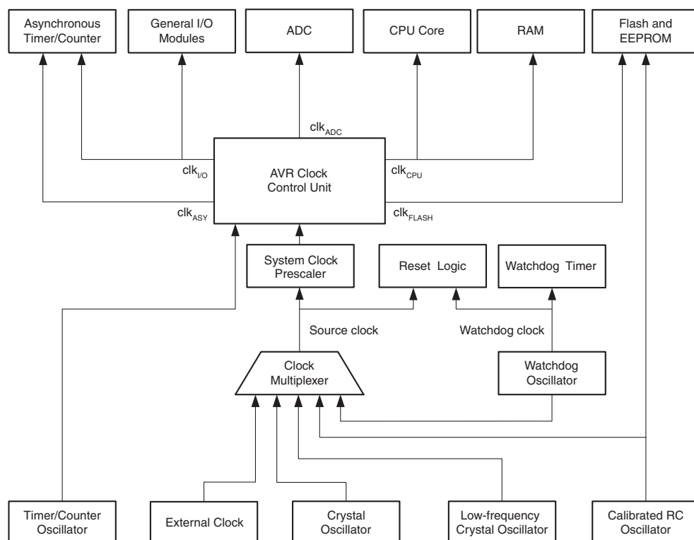
Figure 8-1. Clock Distribution
