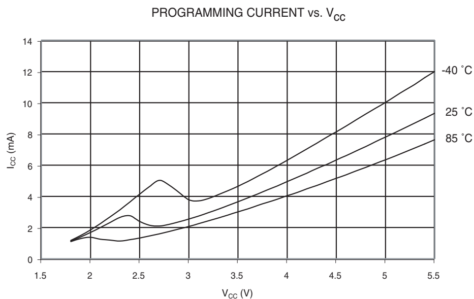
Figure 29-48. Programming Current vs. V_{CC}
