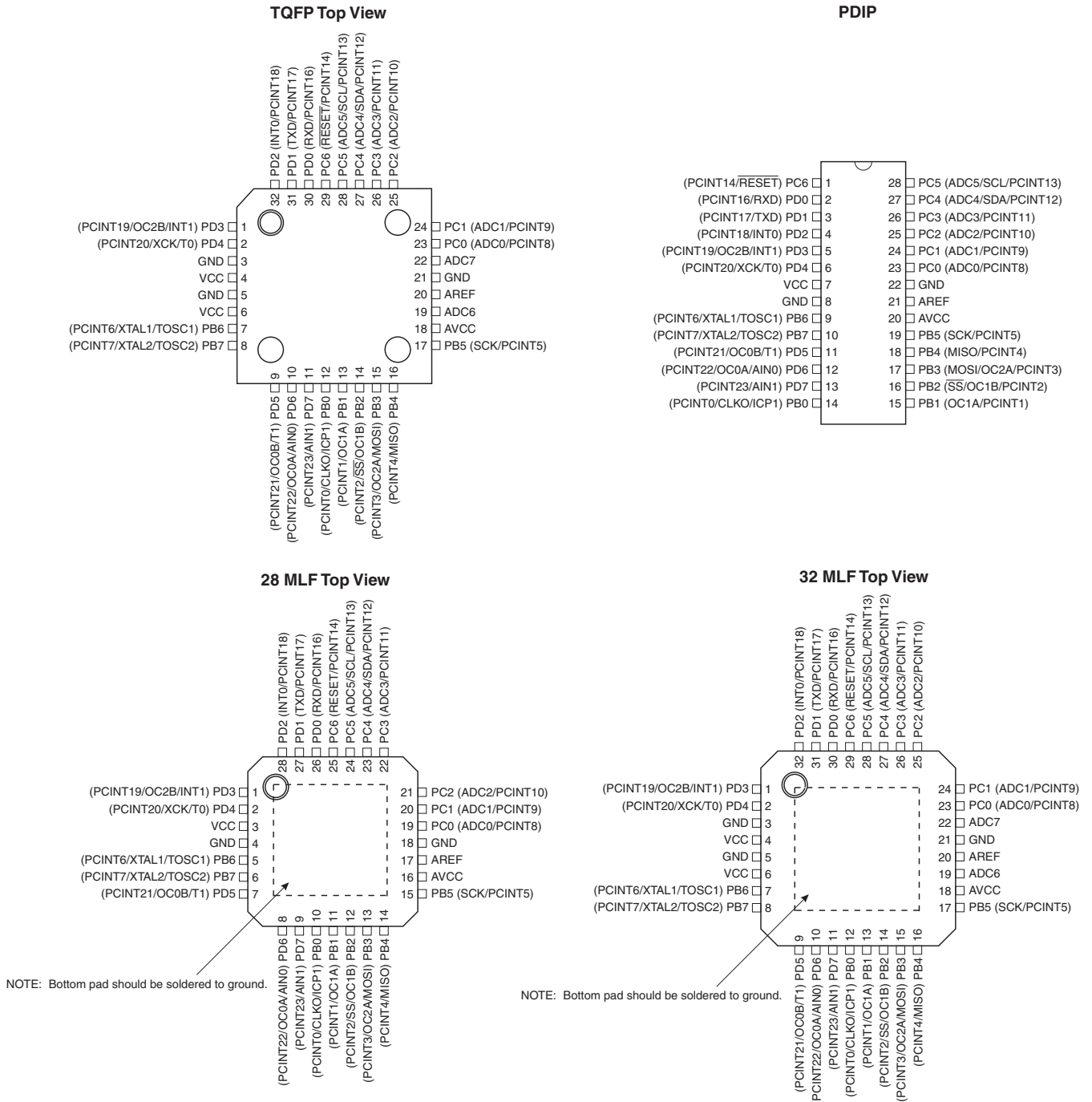
Figure 1-1. Pinout ATmega48/88/1682545RS
