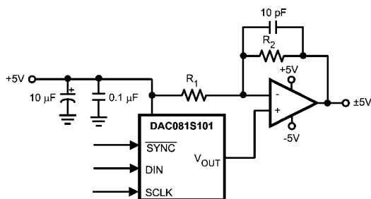
FIGURE 13. Bipolar Operation
