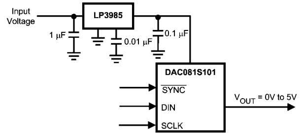
FIGURE 11. Using the LP3985 regulator
