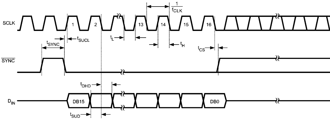
FIGURE 2. DAC081S101 Timing
