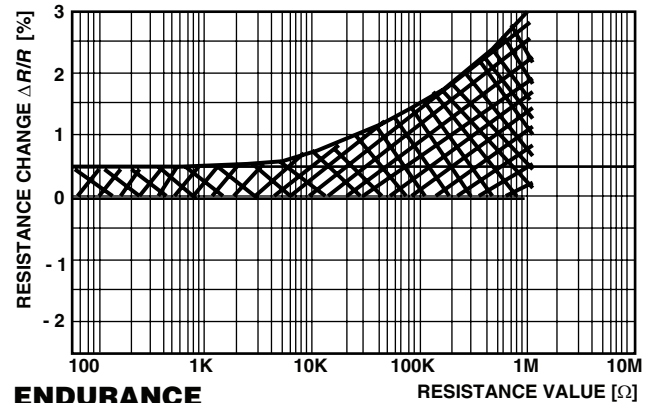
ENDURANCE
