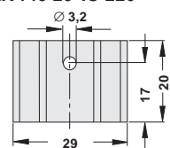
SK 145 20 TO 220
