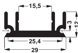
SK 145 20 TO 220
