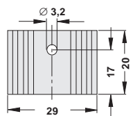
SK 09 20 TO 220
