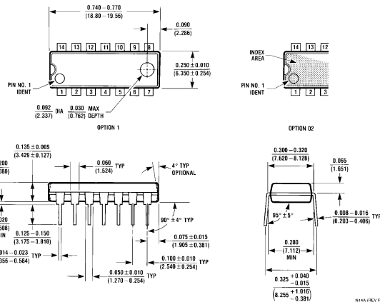
Molded Dual-In-Line Package (N) Order Number CD4093BM or CD4093BCN NS Package Number N14A
