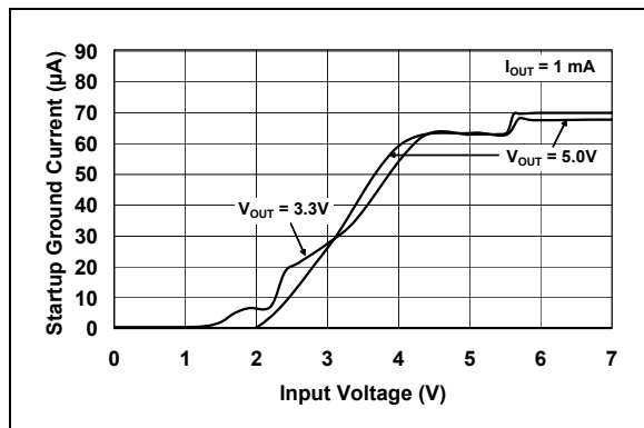
FIGURE 2-25: Startup Ground Current.
