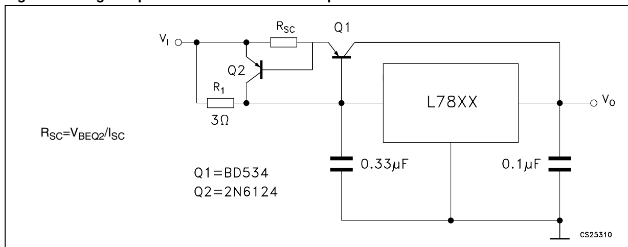
Figure 18. High output current with short circuit protection
