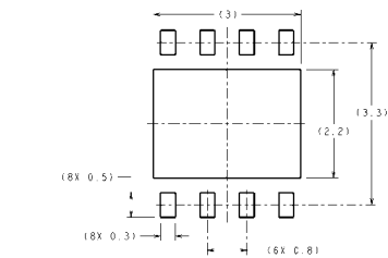
RECOMMENDED LAND PATTERN 1:1 RAT ON WITH PKG SOLDER PADS
