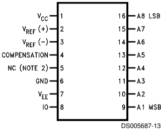
Small-Outline Package
