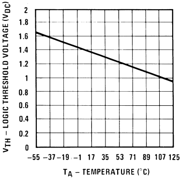
Logic Threshold Voltage vs Temperature
