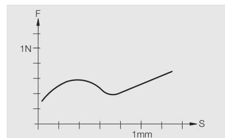
Actuating force / travel diagram
