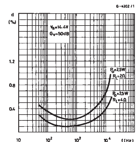
Figure 13 : Distortion versus Frequency (Stereo amplifier)
