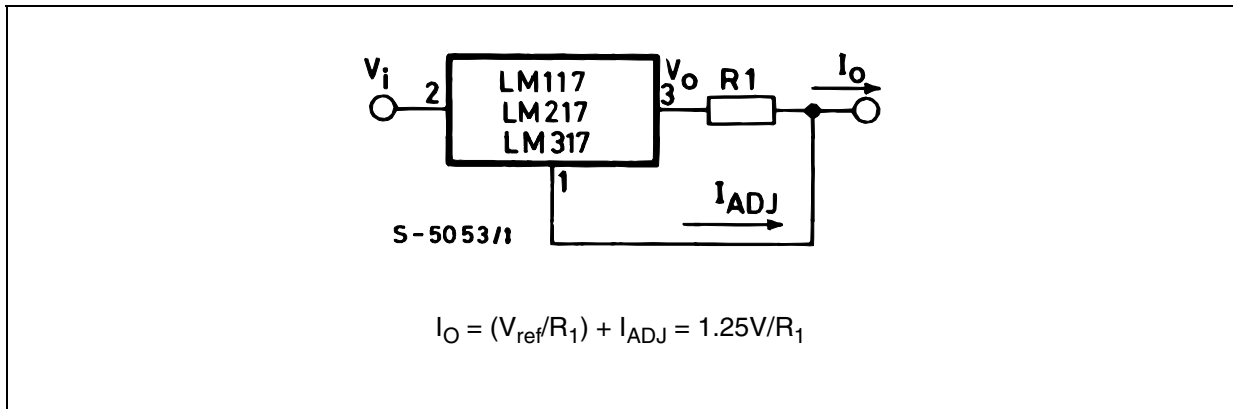
Figure 9. Current regulator
