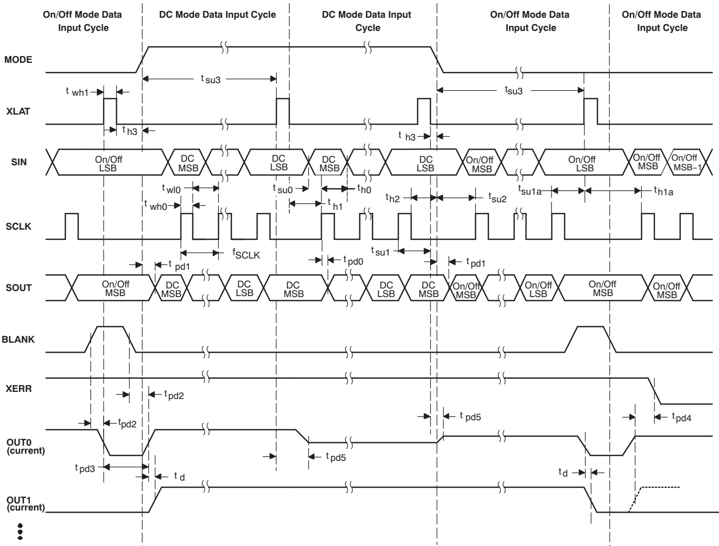
Figure 16. Timing Chart Example for ON/OFF Setting to Dot-Correction
