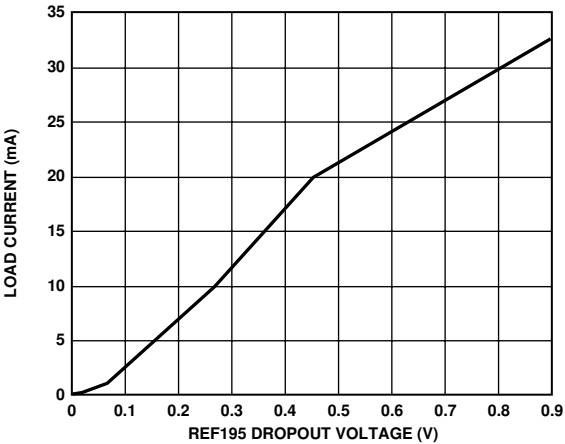
Figure 19. Load Current vs. Dropout Voltage
