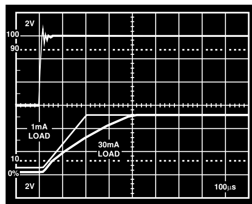
Figure 14. Power On Response Time
