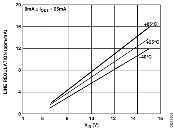
Figure 5. REF195 Line Regulator vs. V_{IN}
