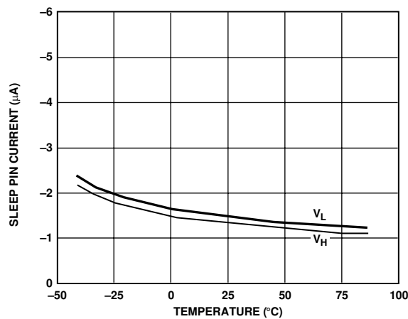
Figure 8. \overline{SLEEP} Pin Current vs. Temperature
