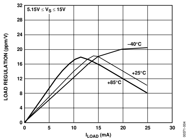
Figure 4. REF195 Load Regulator vs. I_{LOAD}
