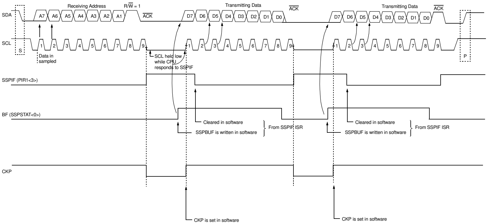
FIGURE 15-9: I 2 C SLAVE MODE TIMING (TRANSMISSION, 7-BIT ADDRESS)
