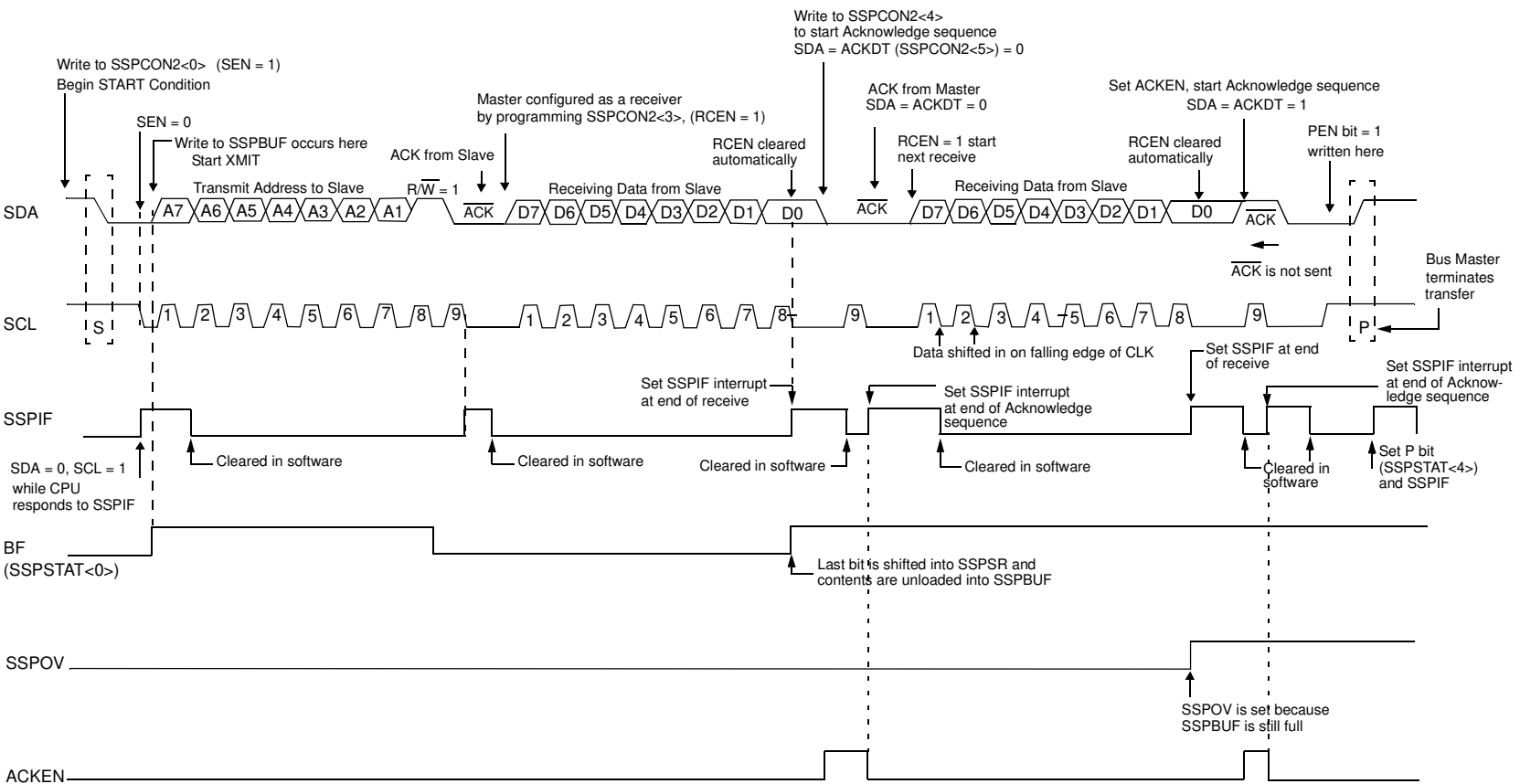
FIGURE 15-22: I 2 C MASTER MODE WAVEFORM (RECEPTION, 7-BIT ADDRESS)
