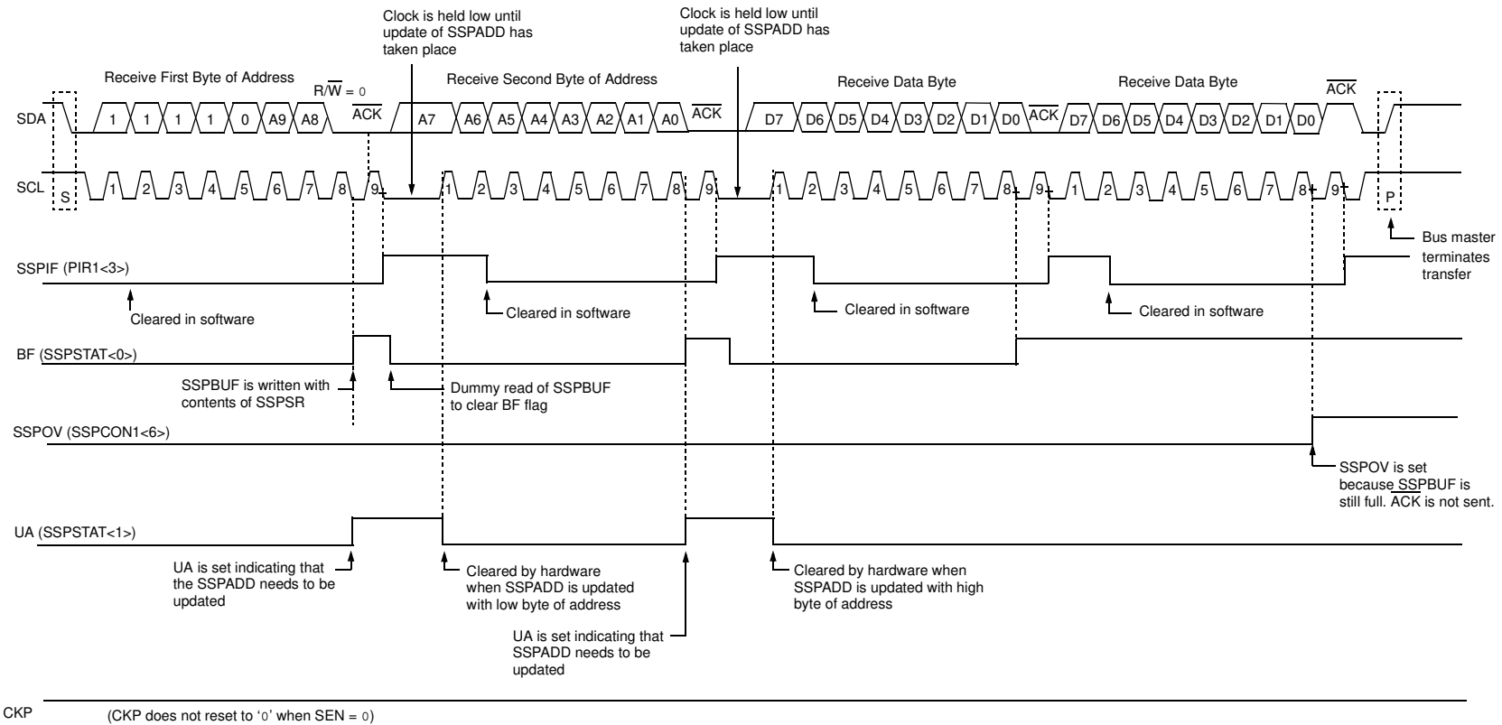
FIGURE 19-10: I 2 C™ SLAVE MODE TIMING WITH SEN = 0 (RECEPTION, 10-BIT ADDRESS)
