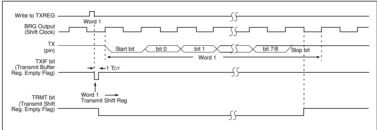
FIGURE 20-4: ASYNCHRONOUS TRANSMISSION
