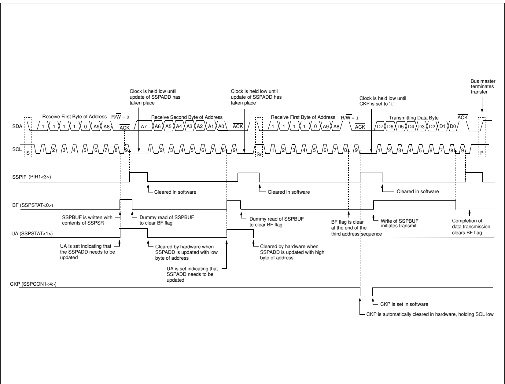
FIGURE 19-11: I 2 C™ SLAVE MODE TIMING (TRANSMISSION, 10-BIT ADDRESS)
