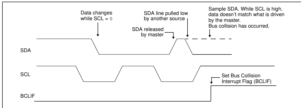
FIGURE 19-25: BUS COLLISION TIMING FOR TRANSMIT AND ACKNOWLEDGE
