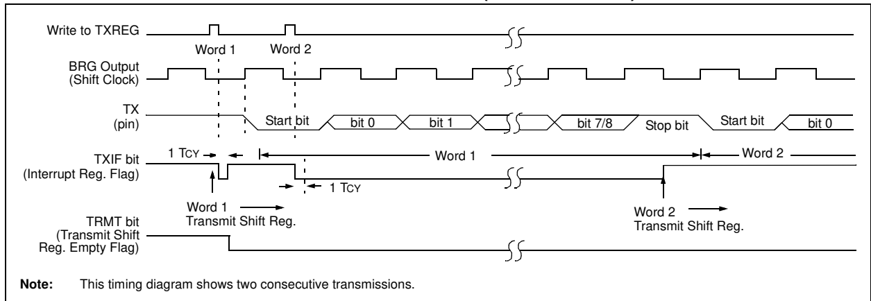
FIGURE 20-5: ASYNCHRONOUS TRANSMISSION (BACK TO BACK)
