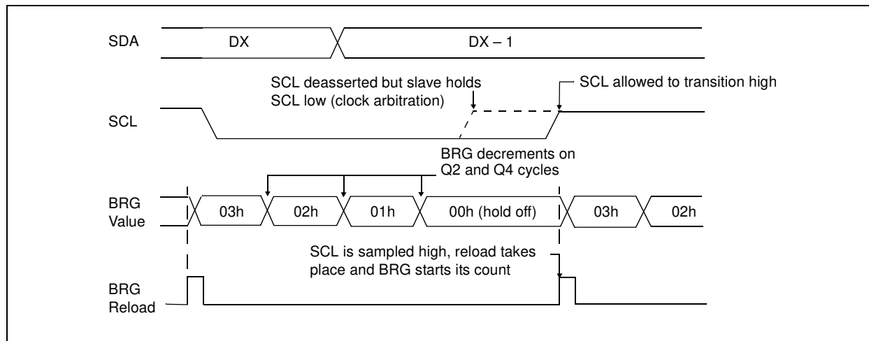
FIGURE 19-18: BAUD RATE GENERATOR TIMING WITH CLOCK ARBITRATION
