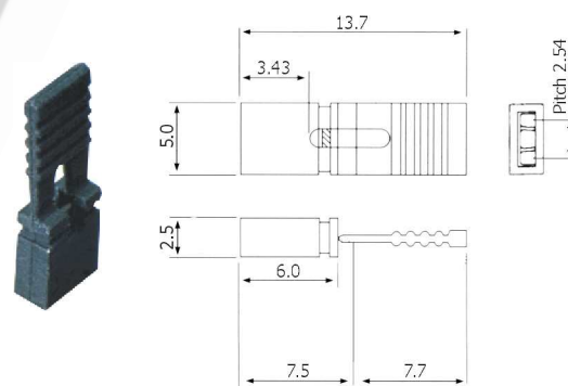
JUMPER-H/B, -H/R:
