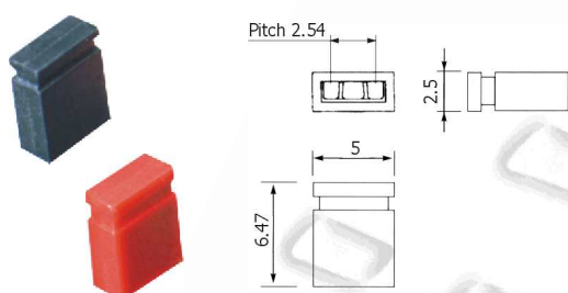
JUMPER-B-Z, -R-Z:
