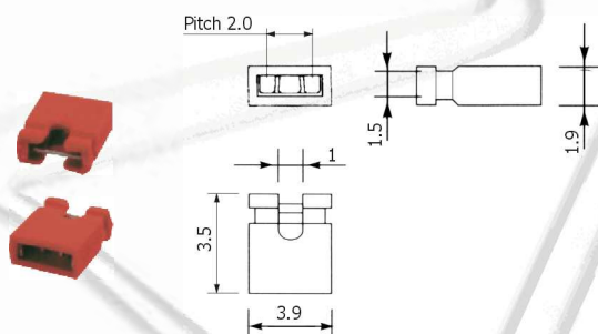
JUMPER-2.0/B, -2.0/R:
