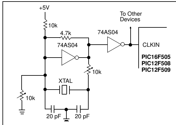
FIGURE 7-3: EXTERNAL PARALLEL RESONANT CRYSTAL OSCILLATOR CIRCUIT
