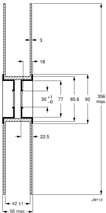
Fig.11 Dimensions of the reel.
